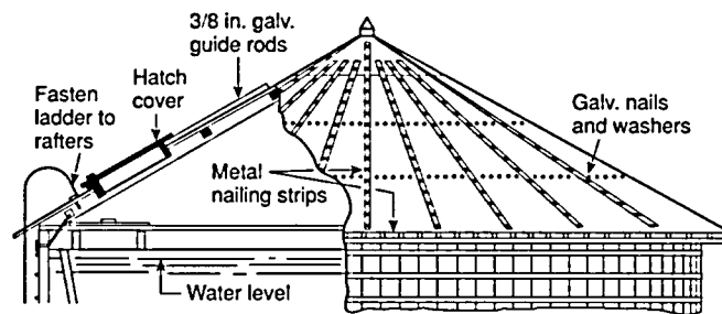
Figure B-4 Section of conical roof.
