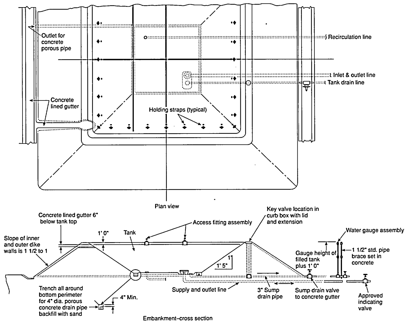
Figure B-5 Typical installation details of an embankment-supported coated fabric suction tank including fittings.
