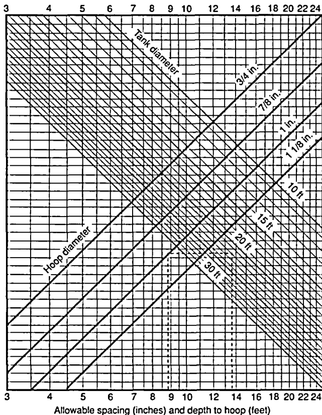
Figure 6-5.3 Hoop spacing diagram for wood tanks.
