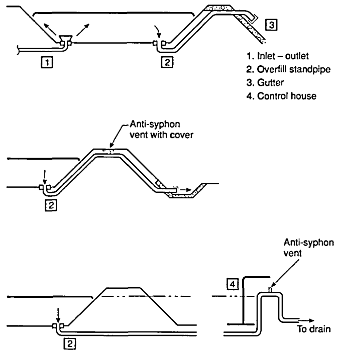
Figure B-8 Embankment-supported coated fabric suction tank overflow standpipe alternates — protect from freezing.
