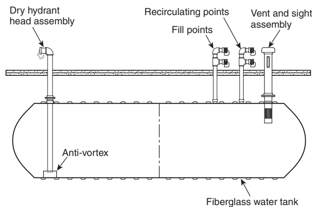
FIGURE A.11.2 Fiberglass Tank as an Underground Cistern.
