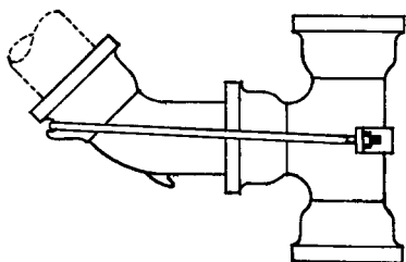
FIG. 96-16. ANCHOR FOR BELL END TEE AND \frac{1}{8} BEND SPIGOT END
