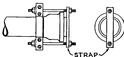
FIG. 96-19. PLUG STRAP FOR BELL END OF PIPE
