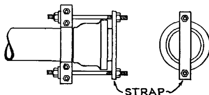
FIG. 96-19. PLUG STRAP FOR BELL END OF PIPE
