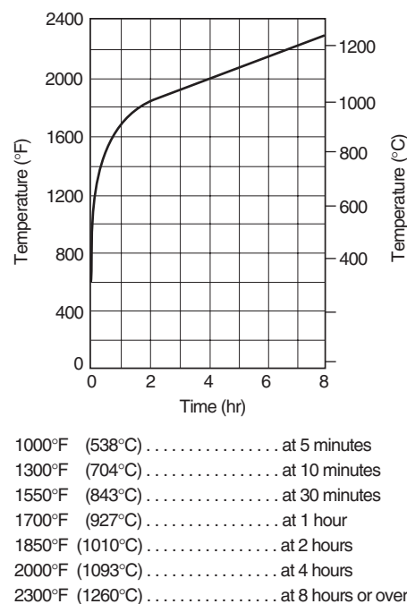
FIGURE 4.1.1 Temperature-Time Curve.
