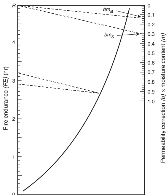
FIGURE F.4 Nomograph for Correcting Fire Endurance for Nonstandard Moisture Content.
