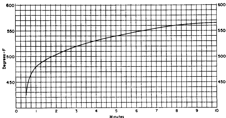
Figure 3. Preheat temperature.
