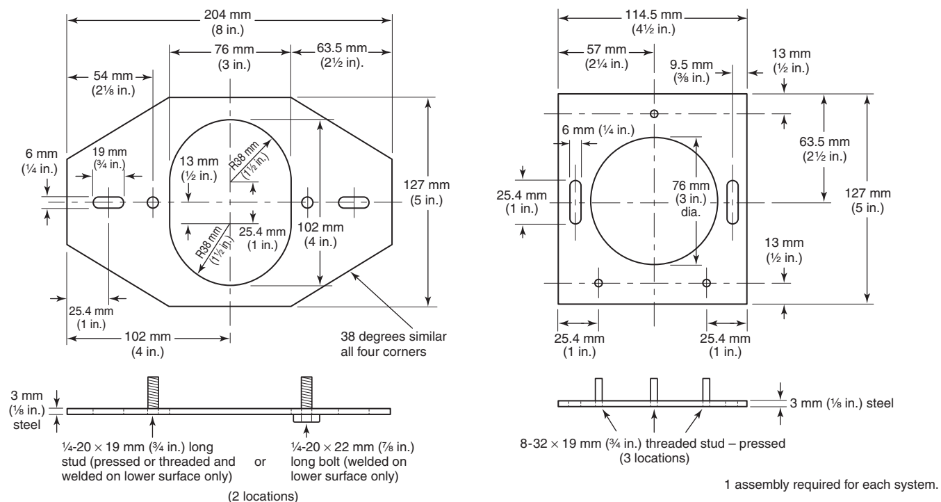
FIGURE C.2(j) Photocell Duct Cross Adjustment Plate.
