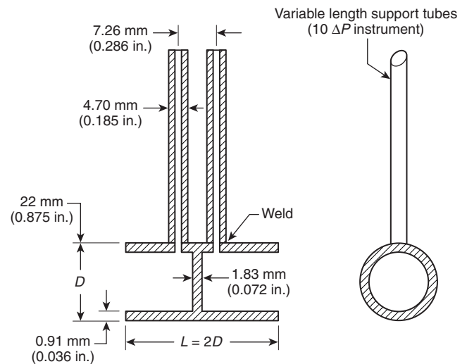
FIGURE 5.4.3 Bidirectional Probe.
