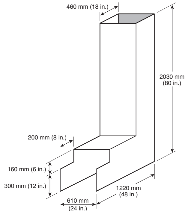
FIGURE 5.1.2 Pipe Chase Interior Dimensions.
