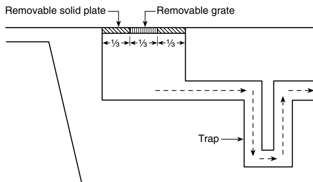
FIGURE A.4.8.5.1(c) Details of drainage trench design.
