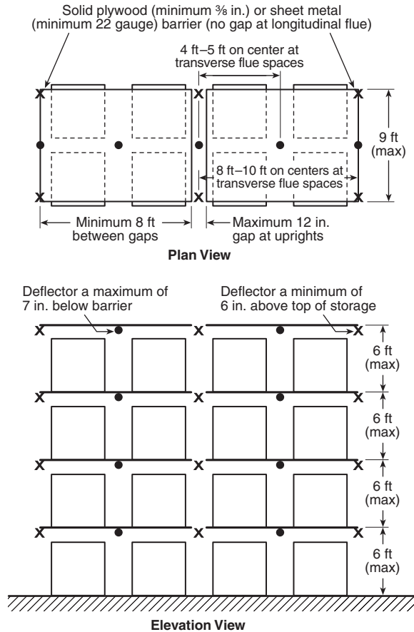
FIGURE 4.8.6.2.1(c) Double-row rack sprinkler layout.
