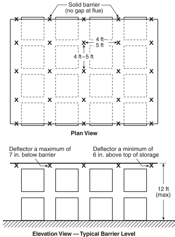
FIGURE 4.8.6.1.1(c) Multiple-row rack sprinkler layout.
