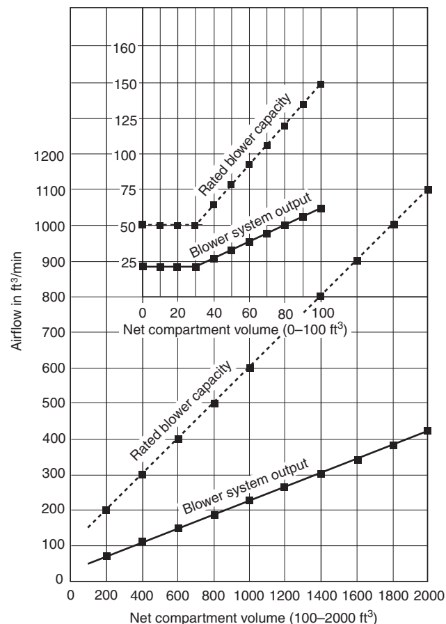
FIGURE 4.5.3.1 Minimum Blower Capacity and System Performance.
