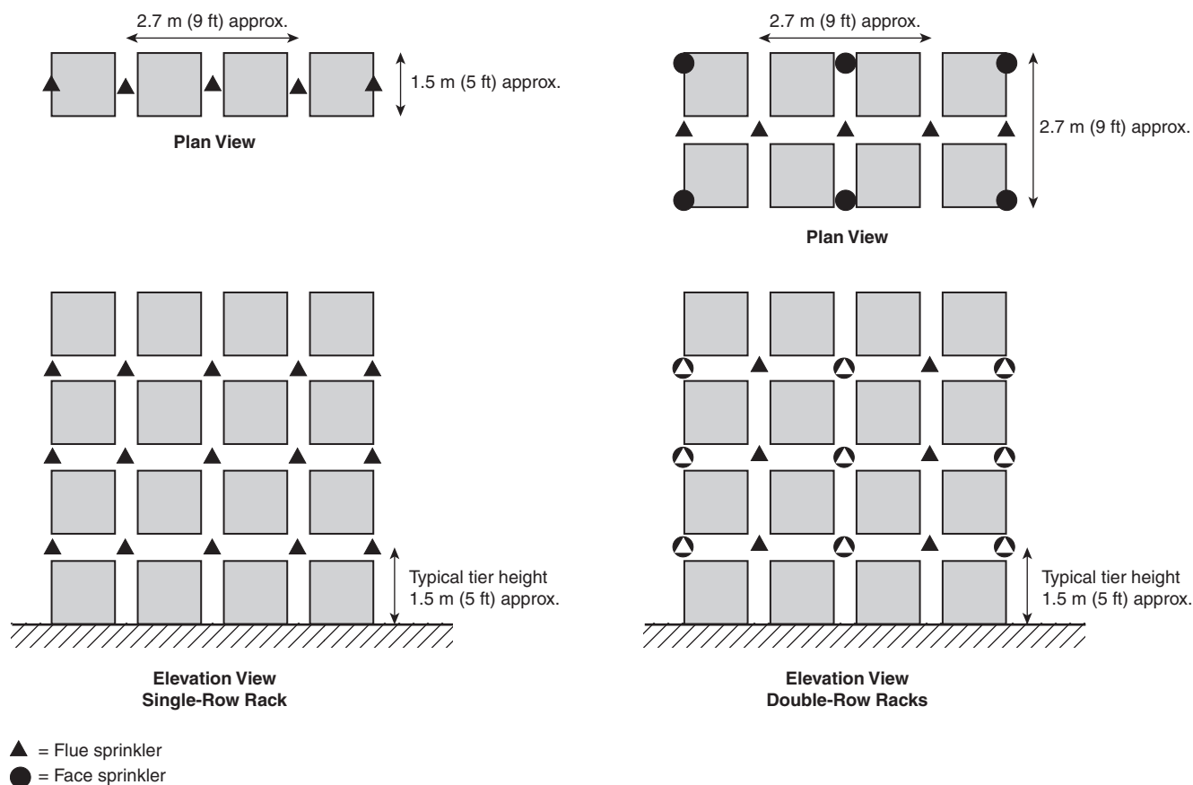
FIGURE 7.4.2.7(d) In-Rack Sprinkler Layout, Uncartoned Level 2 and Level 3 Aerosol Products, Racks up to 6.1 m (20 ft) High Storage.
