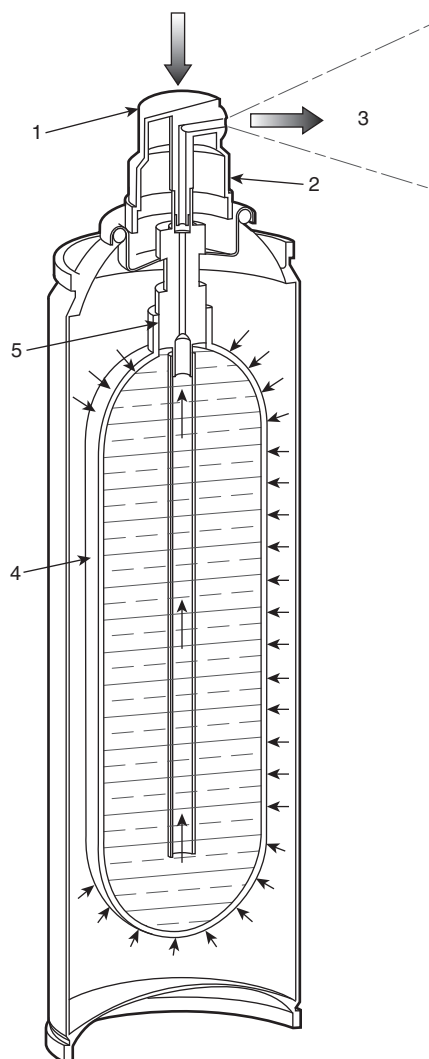
N FIGURE A.3.3.13 One Type of Compartmented Aerosol Container (Cutaway View) with Bag-On-Valve (BOV).
