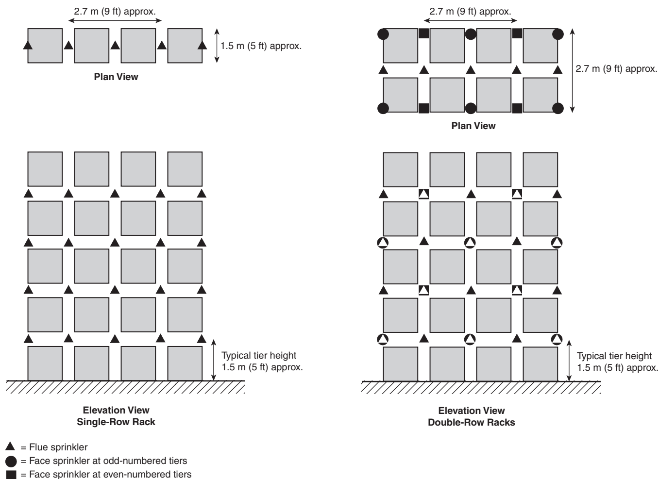
FIGURE 7.4.2.7(e) In-Rack Sprinkler Layout, Uncartoned Level 2 and Level 3 Aerosol Products, Racks up to 7.6 m (25 ft) High Storage.
