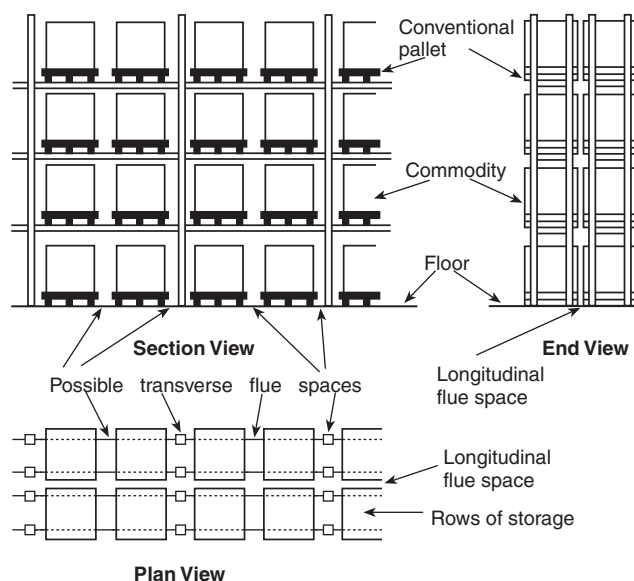
Δ FIGURE A.3.3.26 Typical Double-Row (Back-to-Back) Rack Arrangement. [13:Figure A.3.3.122]
