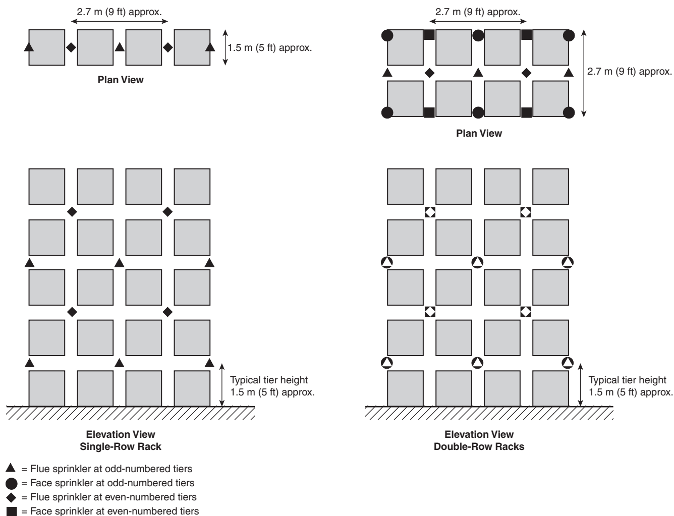
FIGURE 7.4.2.7(b) In-Rack Sprinkler Layout, Cartoned Level 3 Aerosol and Cartoned Plastic Aerosol 2 Products.
