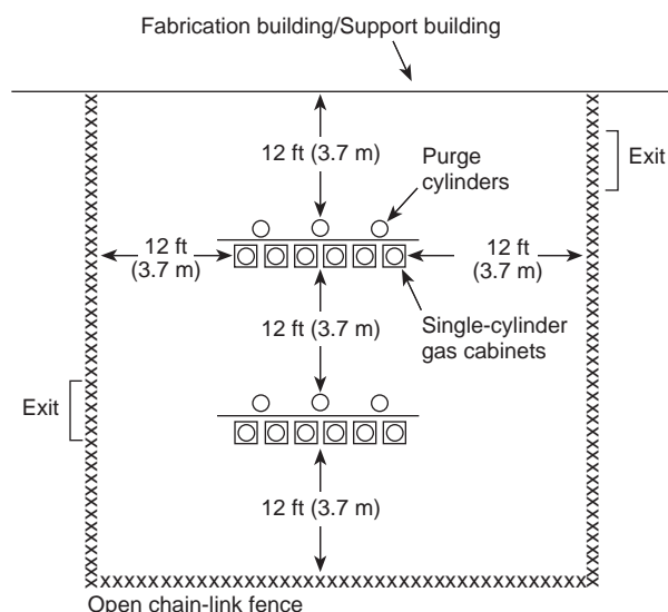
Figure 6-5.3 Silane/toxic mixes dispensing area.
