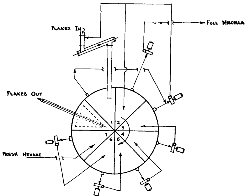
Figure 6. Rotocel Extractor.
