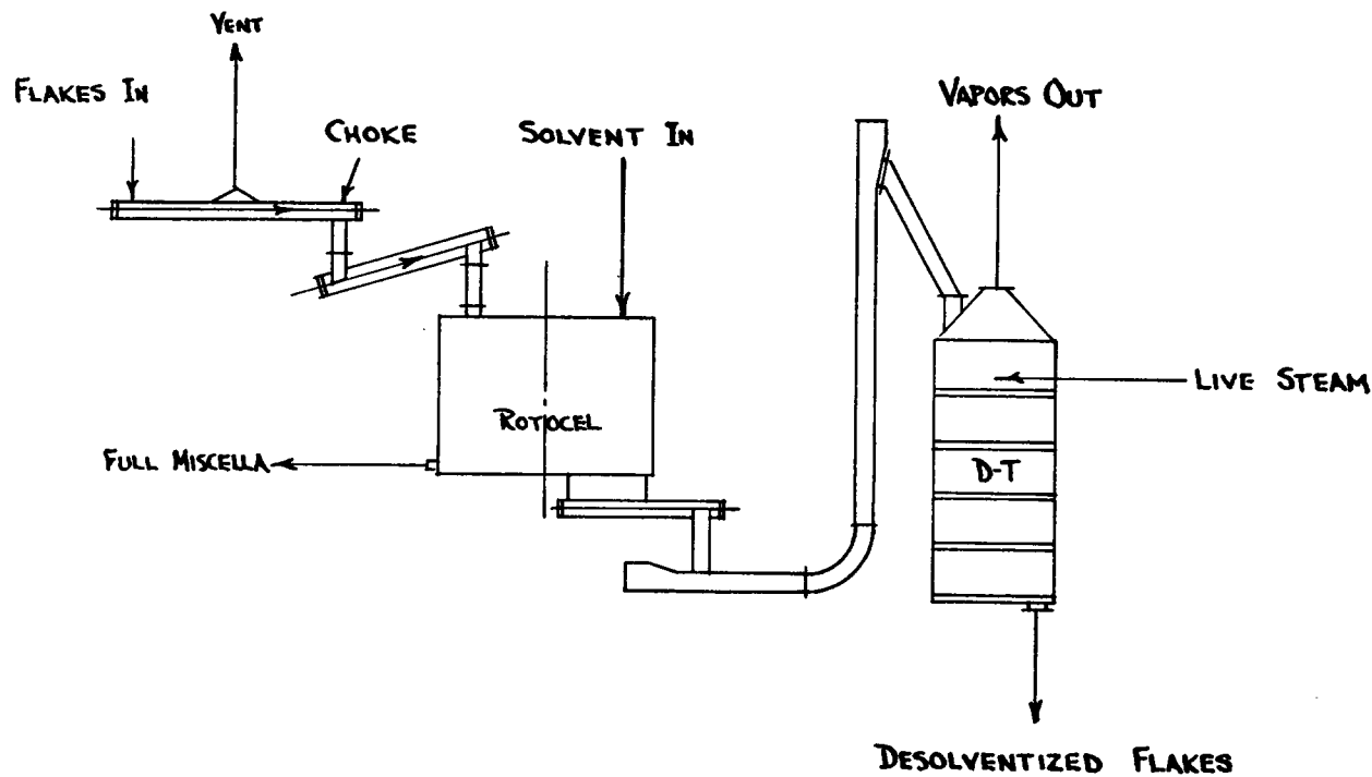
Figure 5. Rotocel System.
