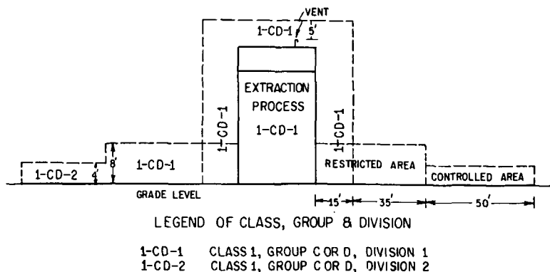
Fig. 1. Type and Extent of Hazardous Areas
