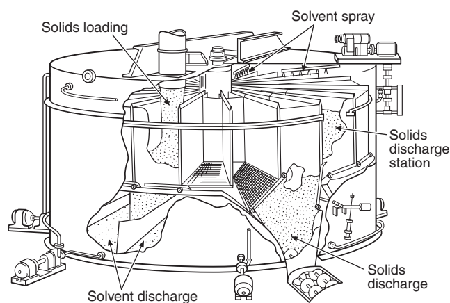
Figure B-3 Rotary or deep bed extractor. (Courtesy Chemical Engineering , Vol. 57, No. 8, August, 1950, p. 109.)
