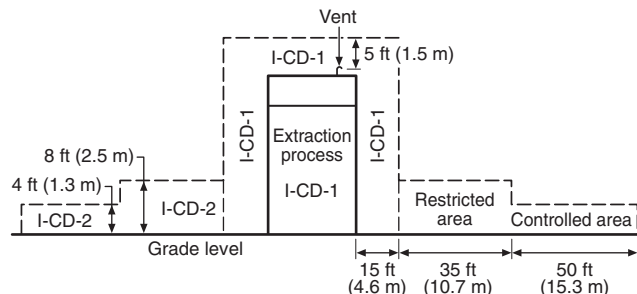
Figure 5-5.2 Type and extent of hazardous areas.
