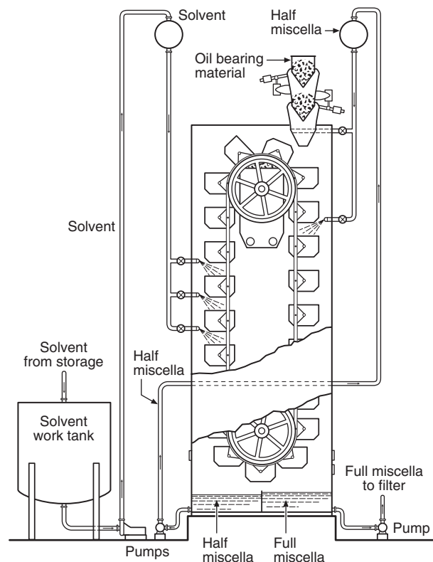
Figure B-2 Vertical basket extractor.
