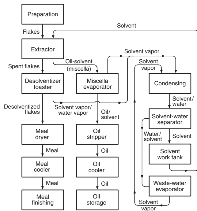
Figure B-1 Flow diagram of extraction process.
