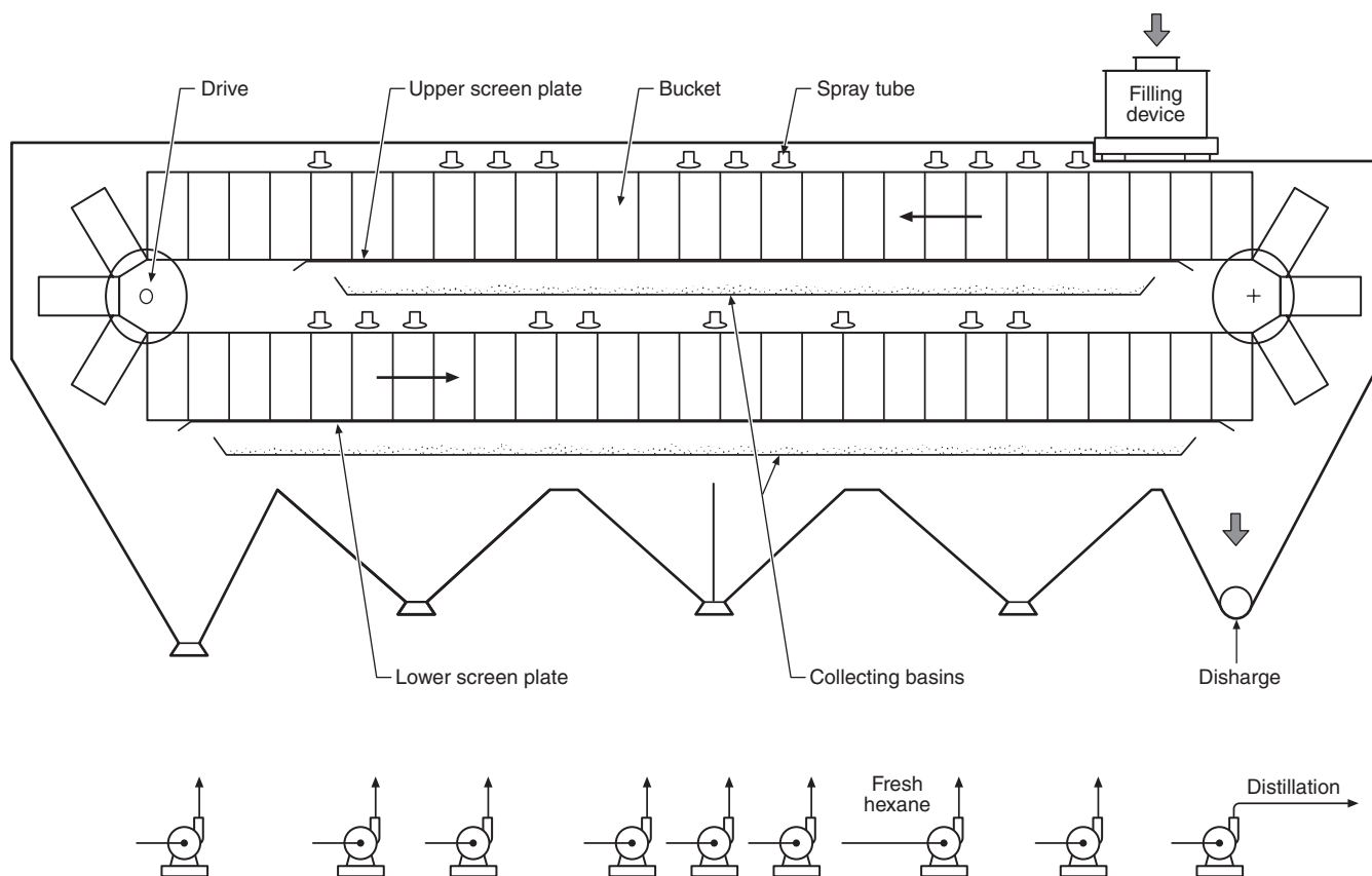
Figure B-7 Sliding cell extractor.
