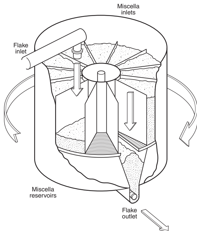
Figure B-5 Stationary-bottom or sliding-plate extractor.
