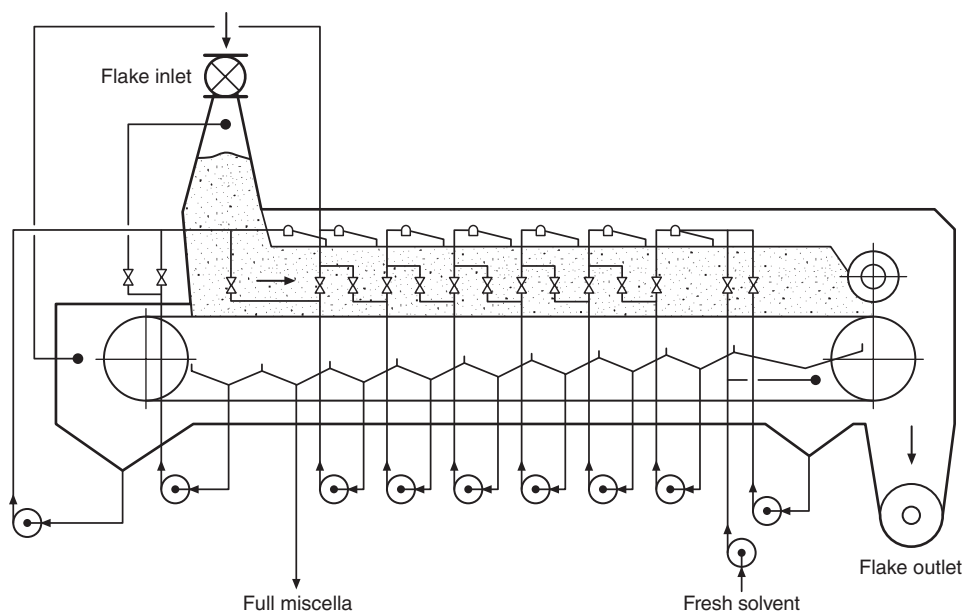
Figure B-6 Perforated belt extractor.
