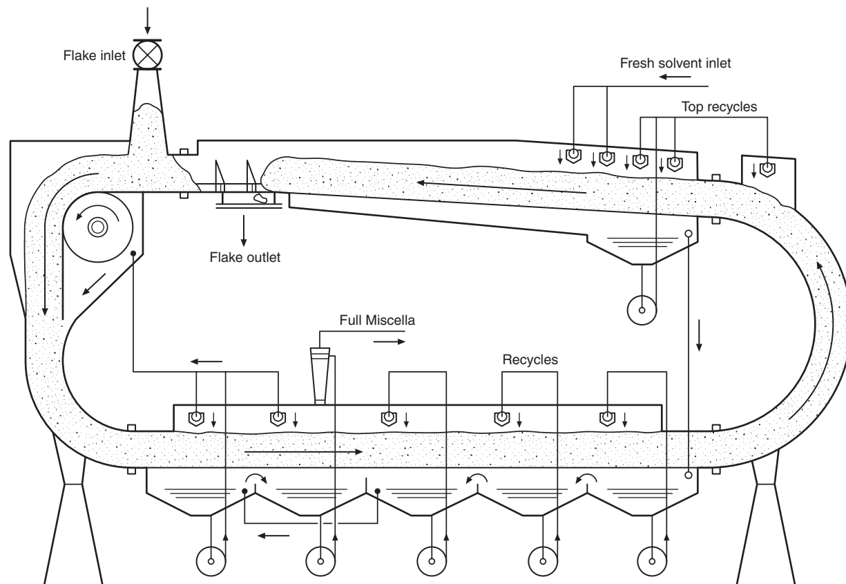
Figure B-8 Rectangular loop extractor.
