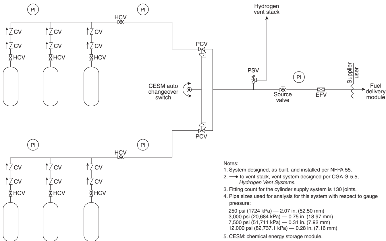
FIGURE A.3.3.11(e) Typical Chemical Energy Storage Model (CESM).
