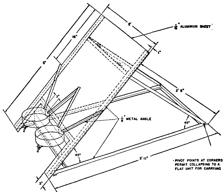
Figure 1. Foam Collector
