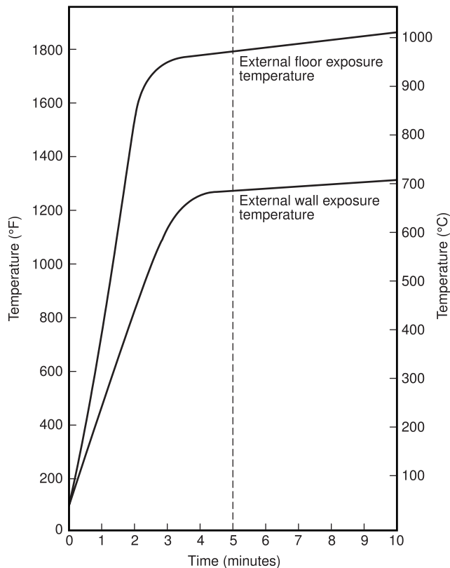
FIGURE 6.4.2 Typical Furnace Time-Temperature Curves for Fire Testing of Aircraft Loading Walkways. (See also Table 6.4.2.)
