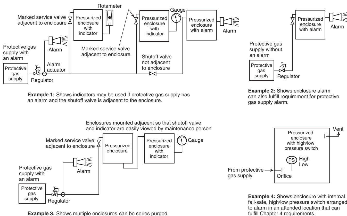
FIGURE A.4.8 Typical Alarm and Indicator Configurations for Types Y and Z Pressurizing. Purge outlet devices that could be provided are not shown for clarity.
