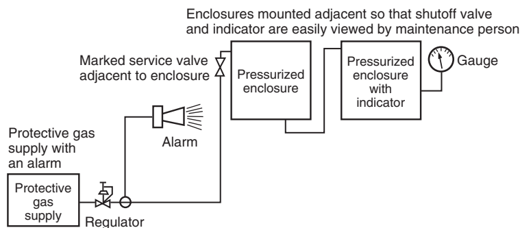
Example 3: Shows multiple enclosures can be series purged.
