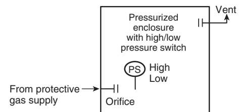
Example 4: Shows enclosure with internal fail-safe, high/low pressure switch arranged to alarm in an attended location that can fulfill Chapter 4 requirements.
