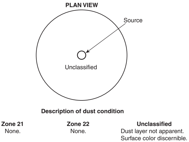
FIGURE 6.10(n) Zone Group IIIC or IIIB Dust — Storage Area; Bags, Drums, or Closed Hoppers.
