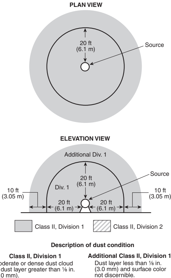
FIGURE 6.10(b) Group E Dust — Indoor, Unrestricted Area; Open or Semi-Enclosed Operating Equipment.
