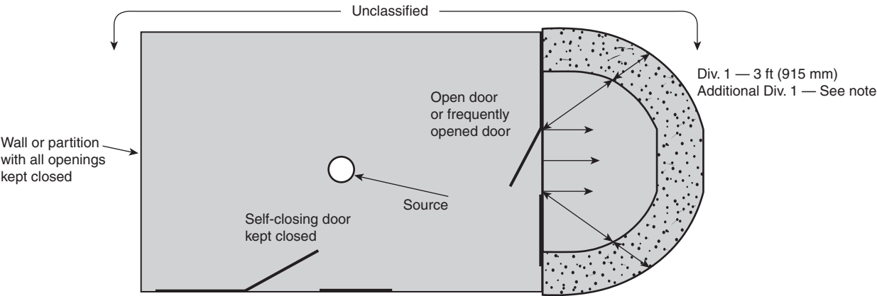
PLAN VIEW
