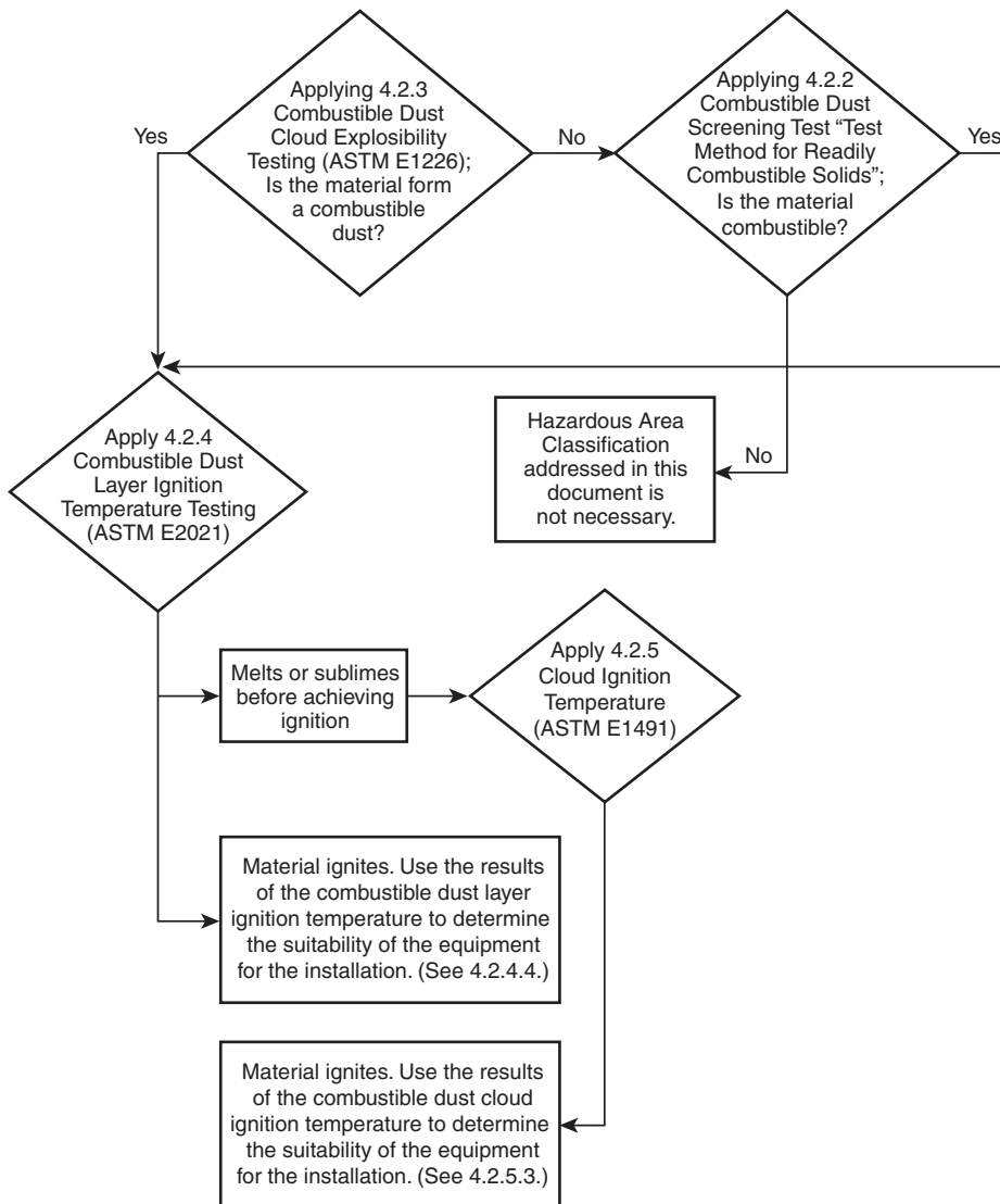
▲ FIGURE 4.2.1 Material Form Testing.
