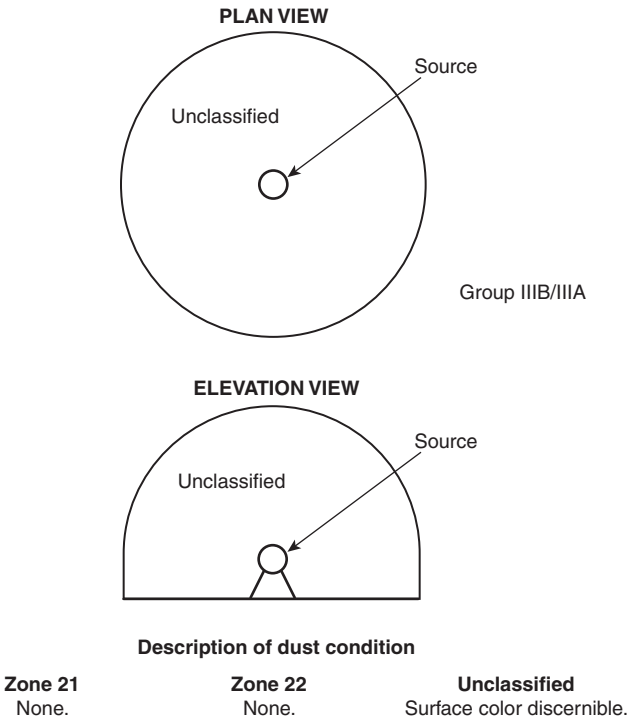
FIGURE 6.10(m) Zone Group IIIB Dust — Indoor, Unrestricted Area; Operating Equipment Enclosed; Area Is an Unclassified Location.
