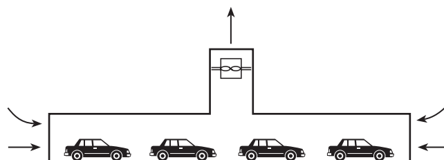
FIGURE H.2.1(d) Longitudinal Ventilation System with Shaft and Central Fans.
