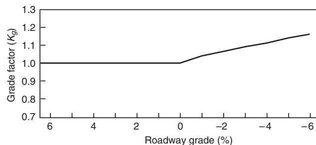
FIGURE C.1 Grade Factor for Determining Critical Velocity.
