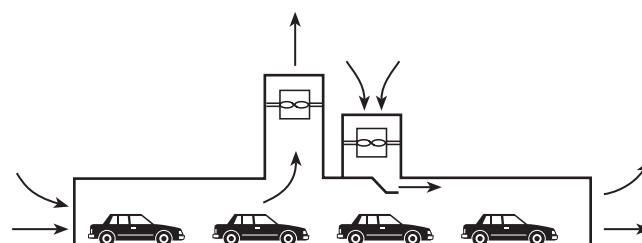
FIGURE H.2.1(c) Longitudinal Ventilation System with Saccardo Nozzle and Shaft.
