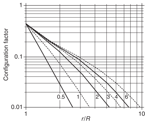
FIGURE 10.3.4.1(b) Configuration Factor for a Horizontal Target and a Vertical Cylindrical Radiator.
