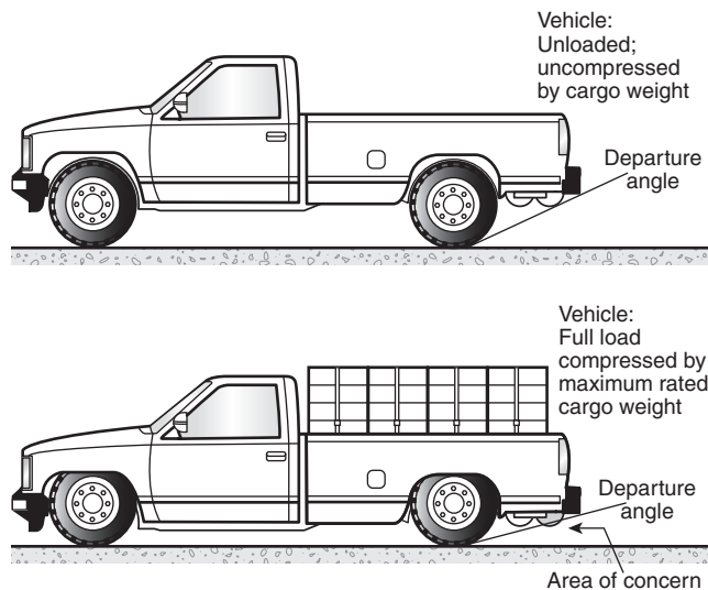
FIGURE 12.4.8 ASME Container Located Behind the Rear Axle.
