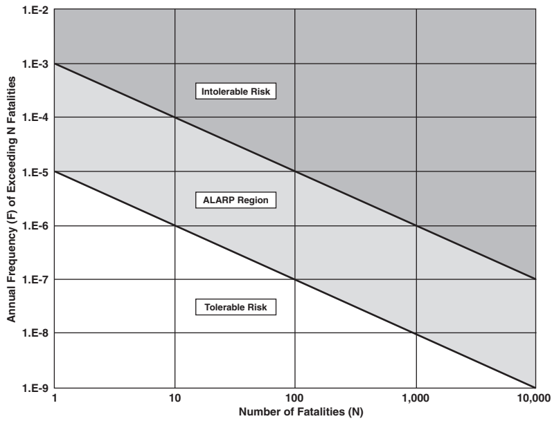
FIGURE 19.10.2(a) Tolerability Regions of Societal Fatality Risk in the F-N Domain.
