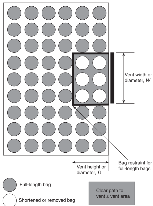
FIGURE A.8.7.1(2)(b) Free Area Normal to Vent for Vertical Filter Elements — Plan View.
