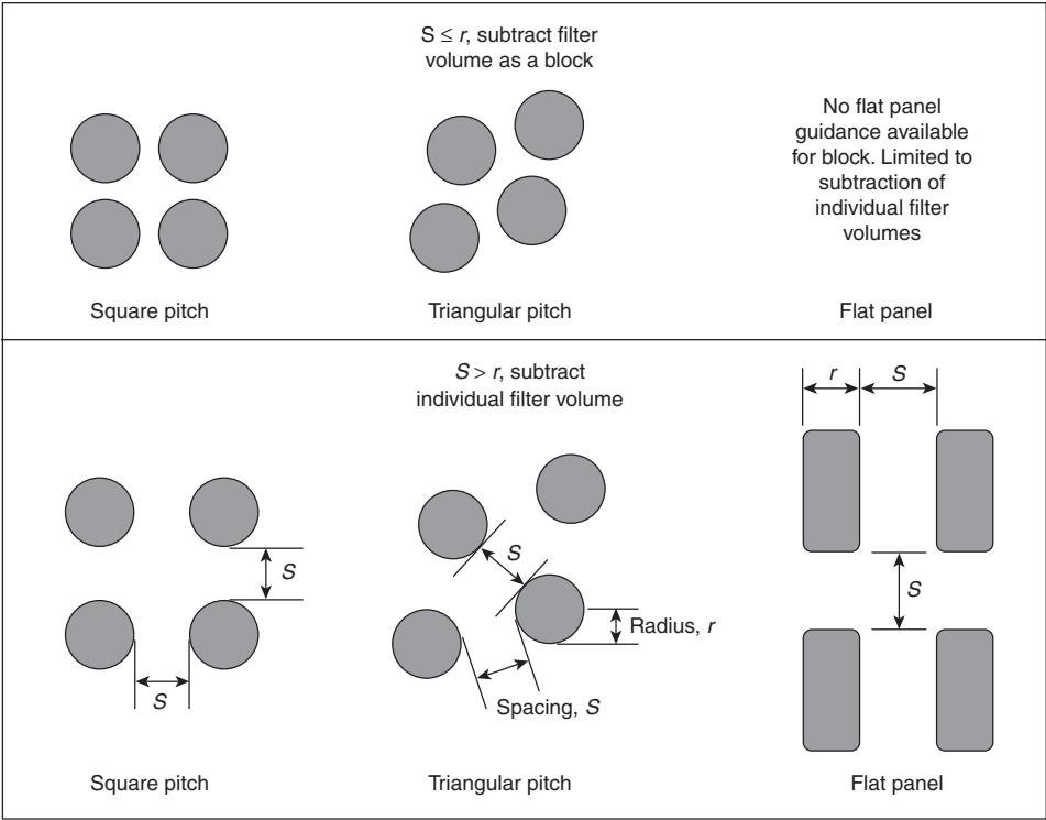
FIGURE 8.7.2 Filter Element Spacing Criteria.
