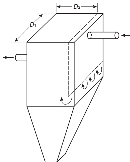
FIGURE A.8.2.5.2 Example of the Cross-Sectional Area of a Complex Enclosure.
