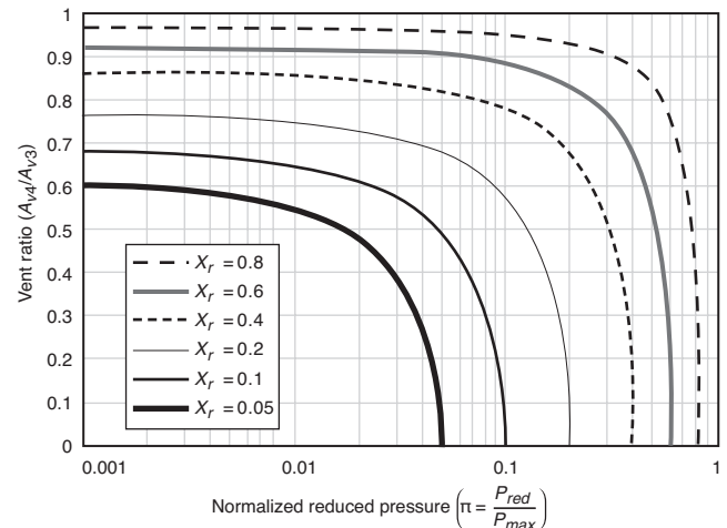
FIGURE A.8.3.2 Partial Volume Vent Area Reduction.
