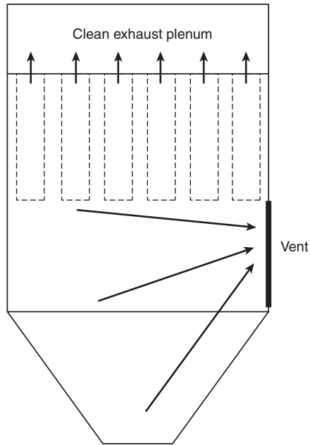
FIGURE A.8.7.1(1)(a) Vent Area Separated from Vertical Filter Elements.
