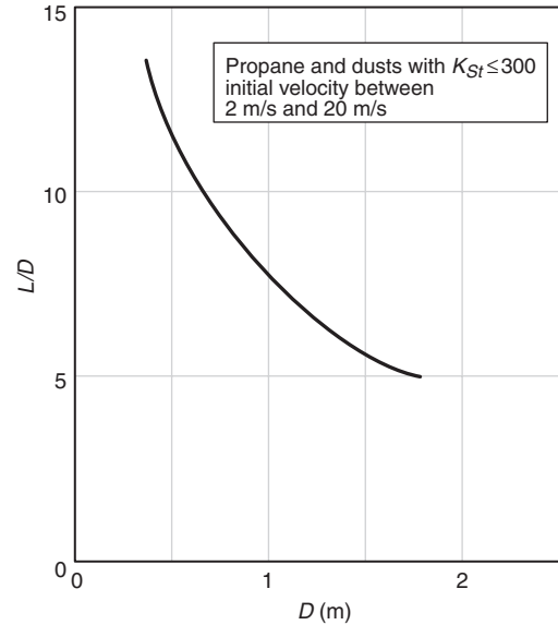
FIGURE 9.3.1 Vent Spacing Needed to Keep P_{red} from Exceeding 0.17 bar for Propane and Dusts with a K_{St} Less Than 300 bar-m/s.
