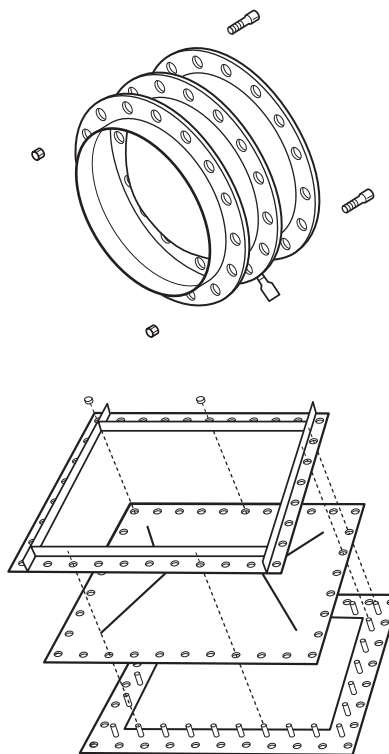
FIGURE A.10.5.2 Typical Rupture Diaphragm.
