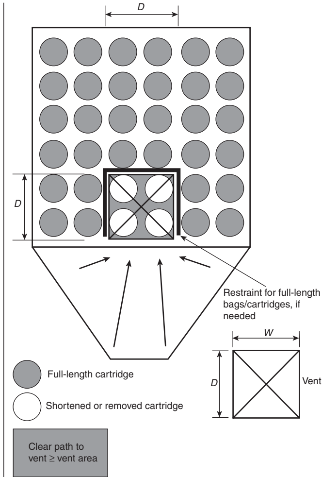
FIGURE A.8.7.1(2)(e) Free Area Normal to Vent for Horizontal Filter Elements — Version 2, End View.
