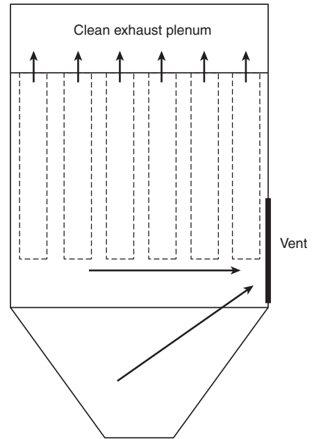
FIGURE A.8.7.3 Insufficient Separation for Vertical Filter Elements.
