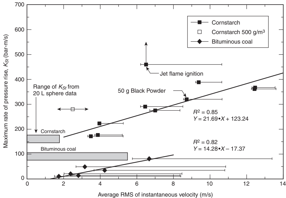
FIGURE A.8.2.5.7 Explosion Severity for Vented Tests in the FMRC 2250 ft 3 Chamber.
