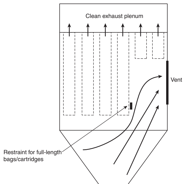
FIGURE A.8.7.1(2)(a) Free Area Normal to Vent for Vertical Filter Elements — Side View.
