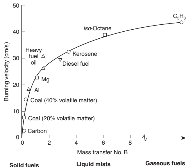
FIGURE A.7.1.2(b) Burning Velocity of Mixtures of Air with Flammable Vapors, Aerosols, or Dusts. (Reprinted from Lees, Lees Loss Prevention in the Process Industries .)
