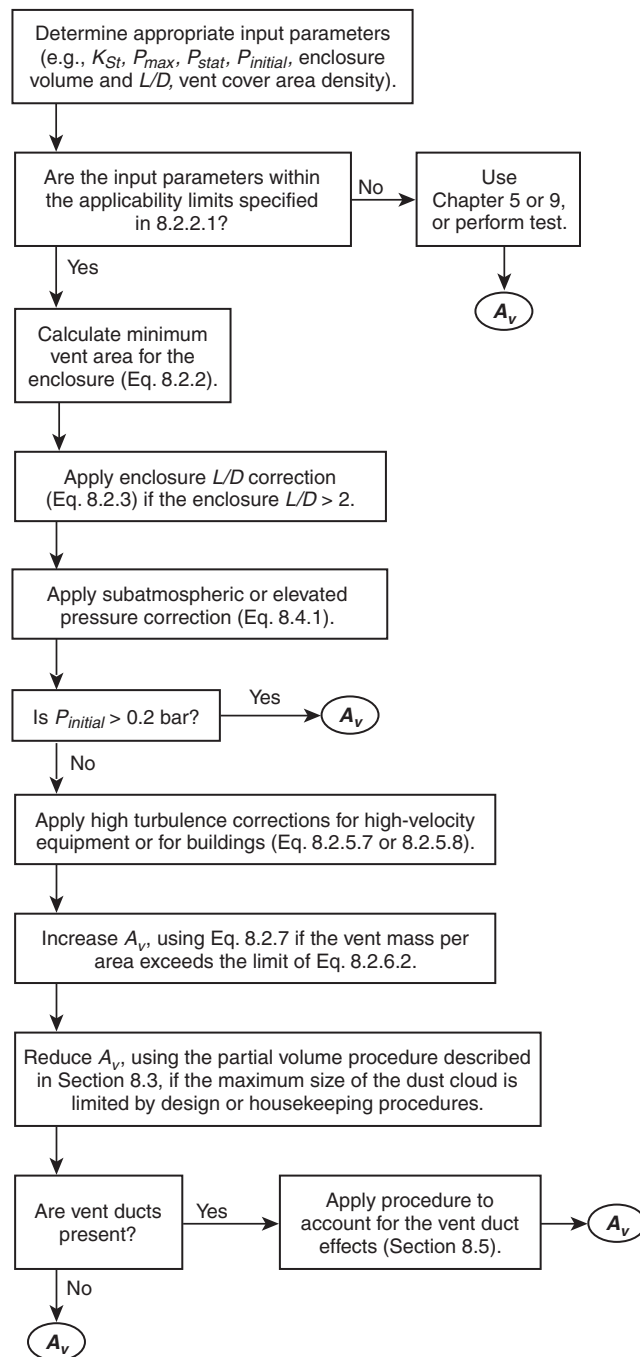
FIGURE 8.1.1.4 Dust Explosion Vent Sizing Calculation Flowchart.
