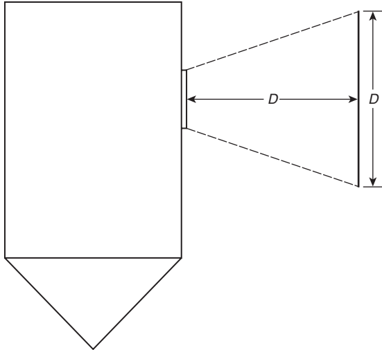
FIGURE 8.9.2.2 Fireball Dimensions.
