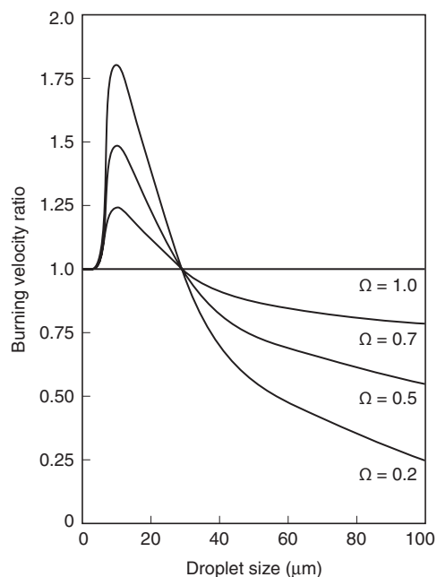
FIGURE A.7.1.2(a) Burning Velocity Predictions Versus Aerosol Droplet Size at Different Values of \Omega .
