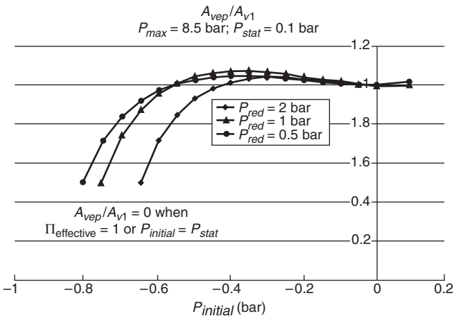
FIGURE A.8.4.2 Typical Effect of Initial Pressure on Required Vent Area.
