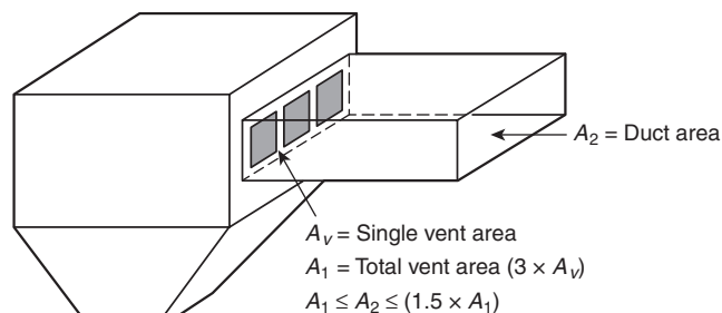
FIGURE 6.8.3 Example Range of Vent Duct Area for Manifolded Vent Duct.
