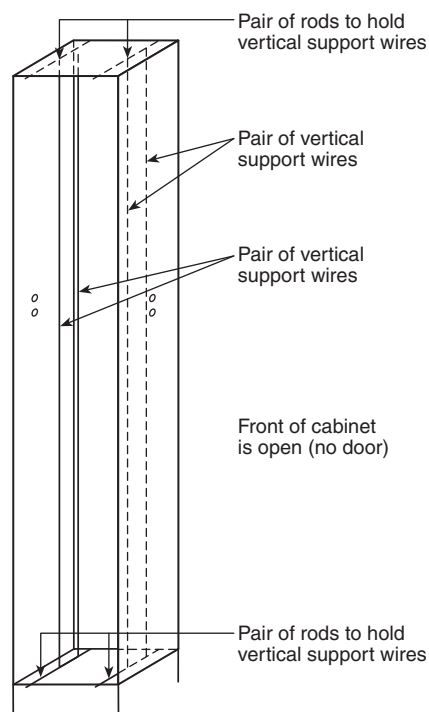
FIGURE 12.2.1.2.3 Vertical Guide Support.
