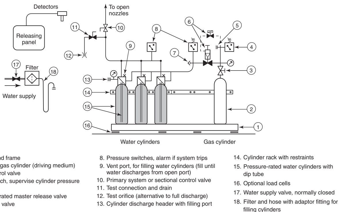
FIGURE A.13.1.6(a) Schematic Representation of a High Pressure, Gas-Driven System with Stored Water (Pre-Engineered System). [Typical]
