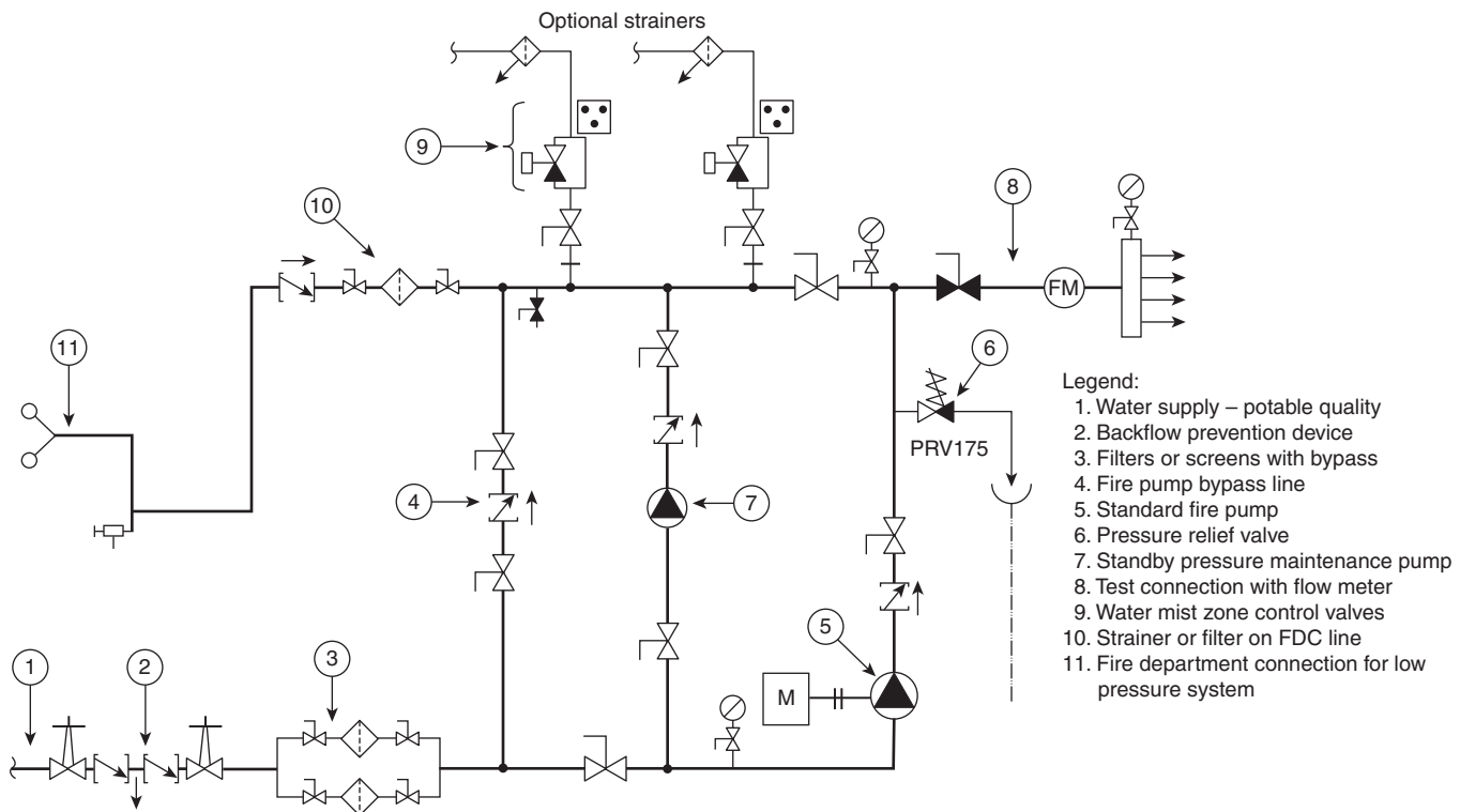
▲ FIGURE A.13.1.6(l) Example of a Piping Arrangement with Fire Department Connection for Low-Pressure Water Mist Systems.
