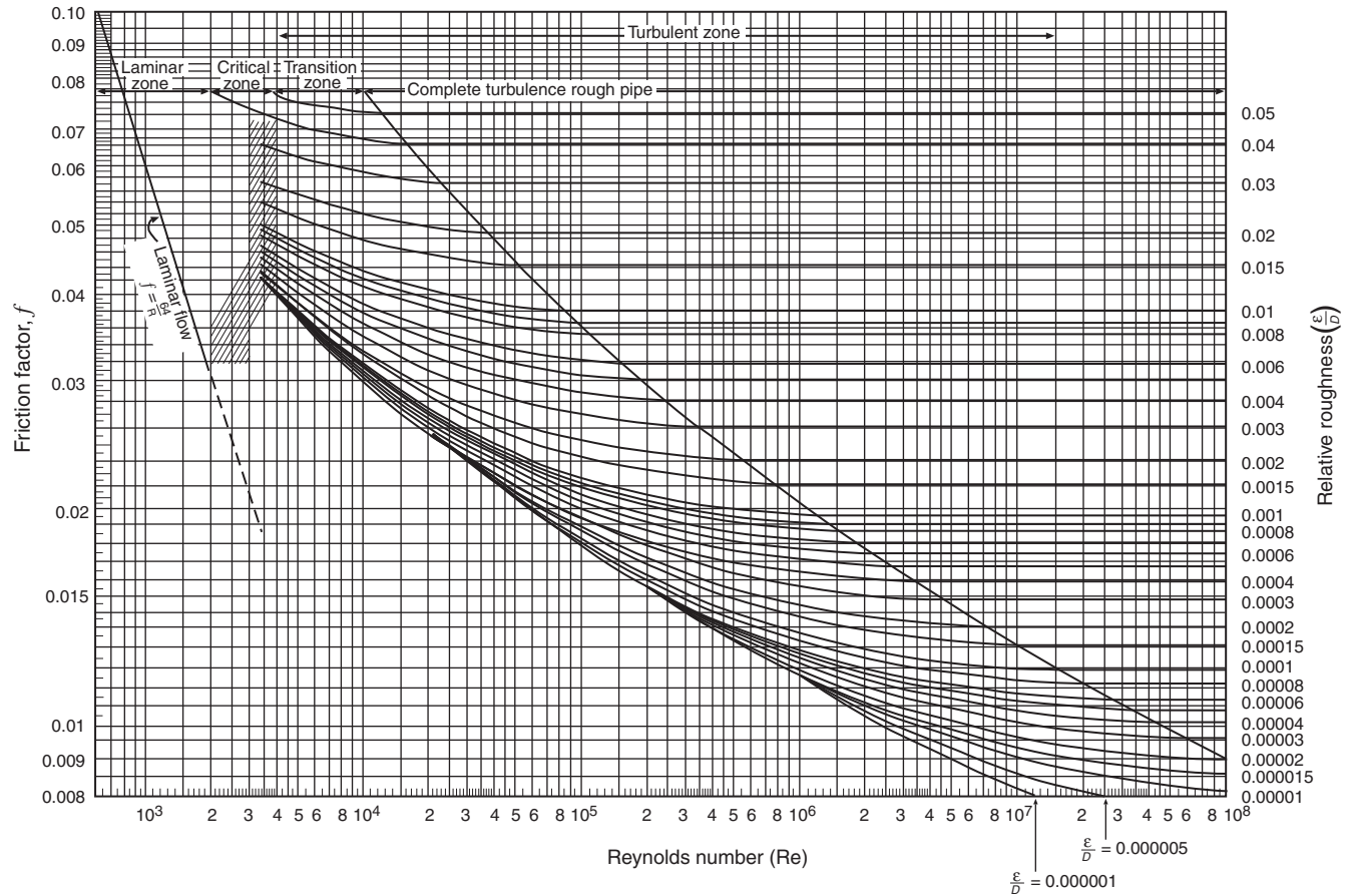
FIGURE 11.2.2 Moody Diagram.
