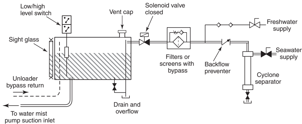
FIGURE A.13.1.6(h) Schematic Diagram of a "Break Tank" Connection in Supply to Positive Displacement Pumps (Marine Systems). [Typical]
