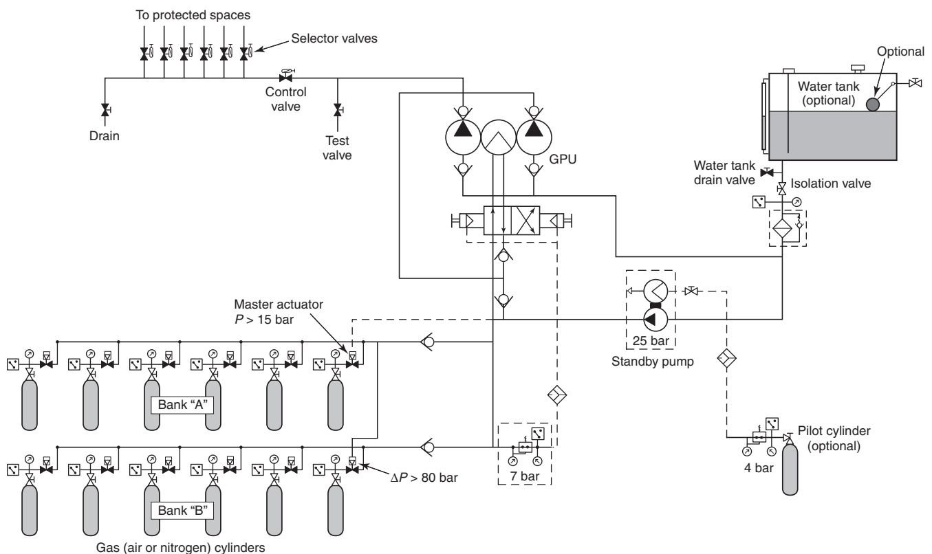
FIGURE A.13.1.6(i) Gas Pump Unit for Machinery Spaces and Gas Turbine Enclosures. [Typical]
