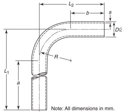
FIGURE A.6.3.6 Installation of Measurements for Application of Table A.6.3.6.
