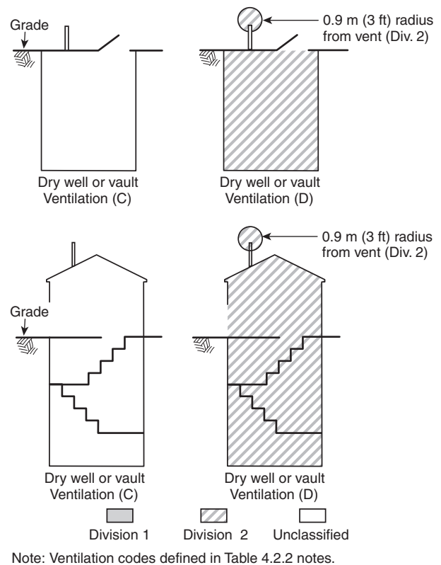
FIGURE A.4.2(d) Belowgrade or Partially Belowgrade Equipment Housing or Vault Physically Separated from Wet Well or Basin; Illustration of Table 4.2.2, Rows 5, 15, 29, and 34.
