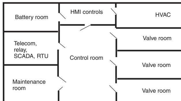
FIGURE 15.3.2.1 Typical Fire Area Separation for Converter Stations.
