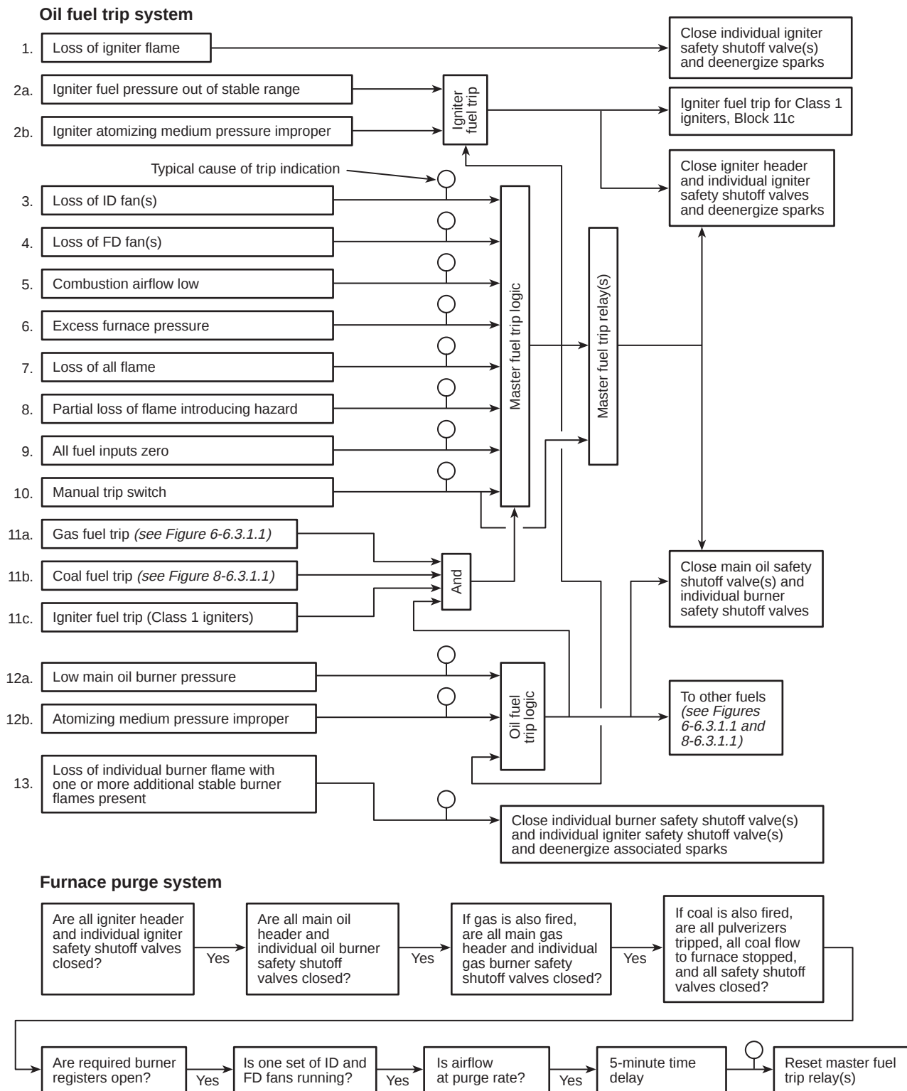
Figure 7-6.3.1.1 Interlock system for oil-fired multiple burner boiler.
