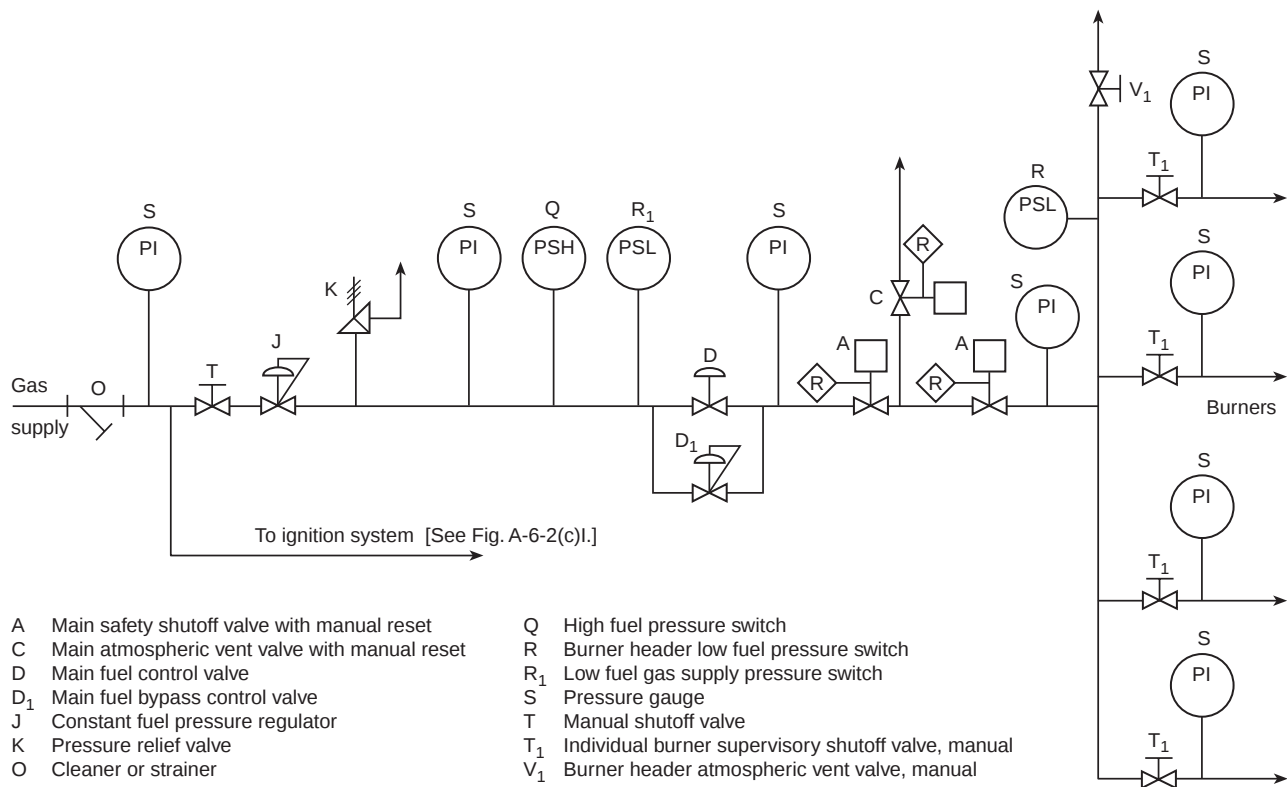
Figure A-6-2(c)II Typical fuel supply system for natural gas-fired multiple burner boiler — manual.
