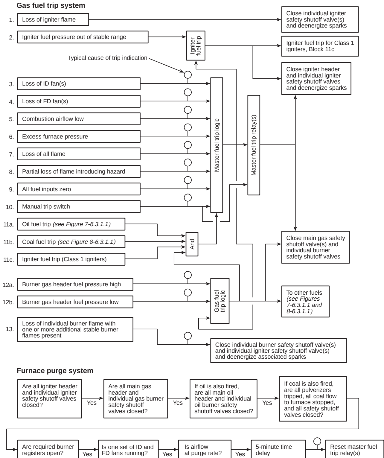
Figure 6-6.3.1.1 Interlock system for natural gas-fired multiple burner boiler.
