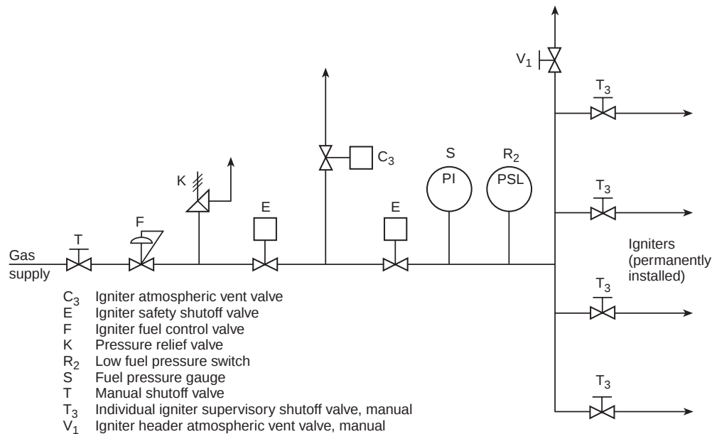
Figure A-6-2(c)I Typical ignition system — manual.
