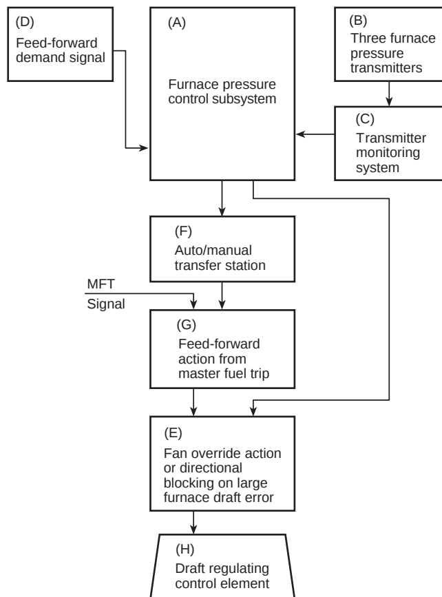
Figure 5-2.2 System requirements.
