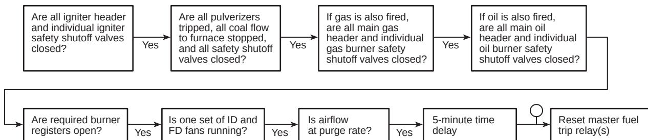
Figure 8-6.3.1.1 Master fuel trip system. Block diagram for furnace interlocks for a pulverized coal-fired multiple burner boiler (see 8-6.3.1).
