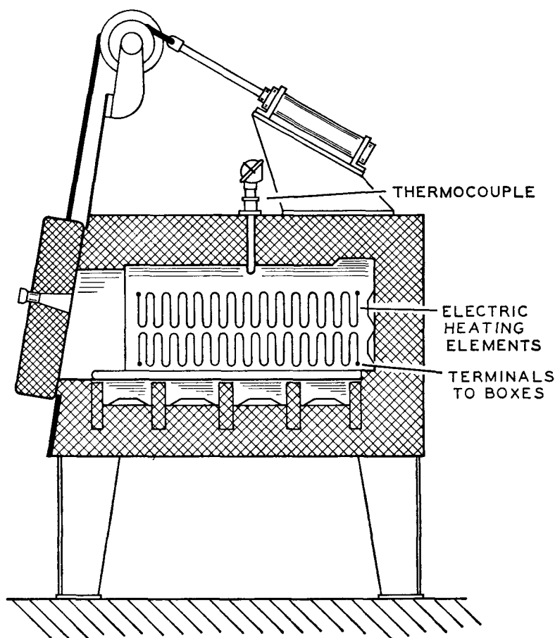
Fig. 5. Electric furnace.
