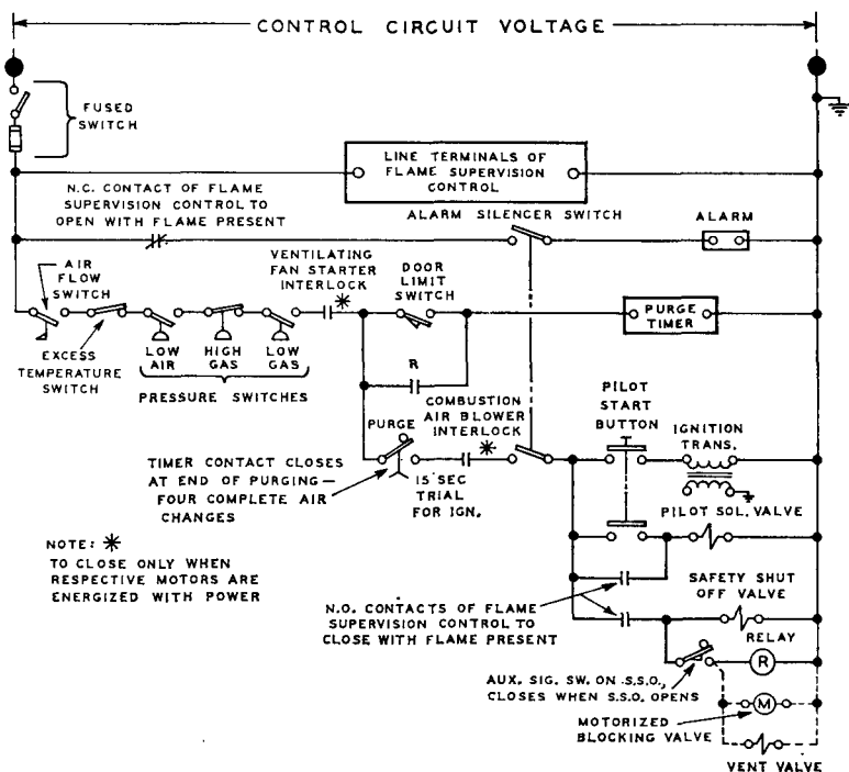
Fig. 1. Typical "ladder-type" schematic diagram
