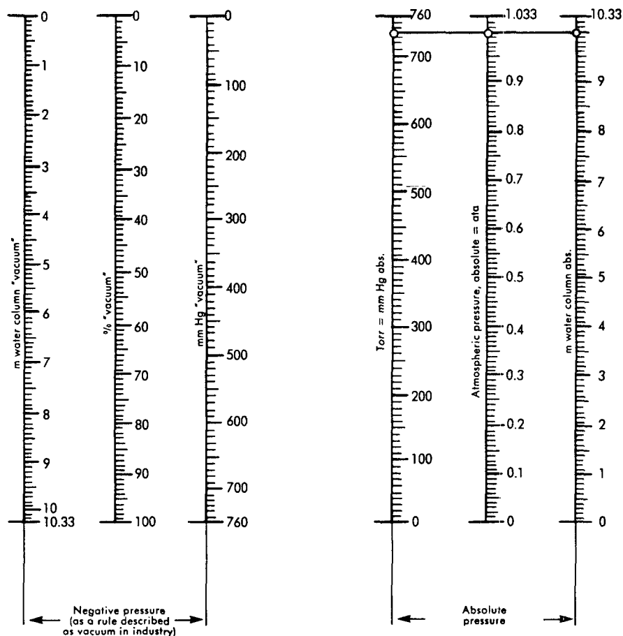
Comparison of Units of Pressure Used in the Rough Vacuum Range
