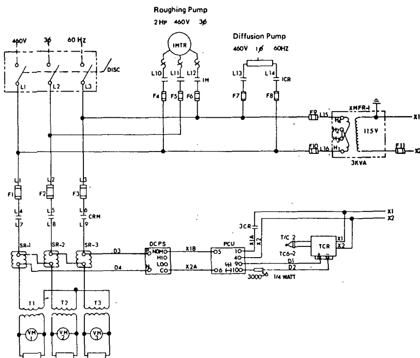
Figure A-1-7(b) Example of Control Wiring Diagram.
