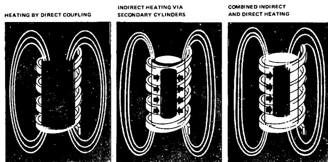
Figure 9-1.1 The Three Induction Heating Methods.
