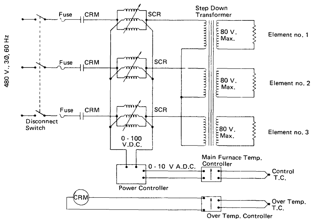
Figure A-3-2.1 Example of Power Supply.
