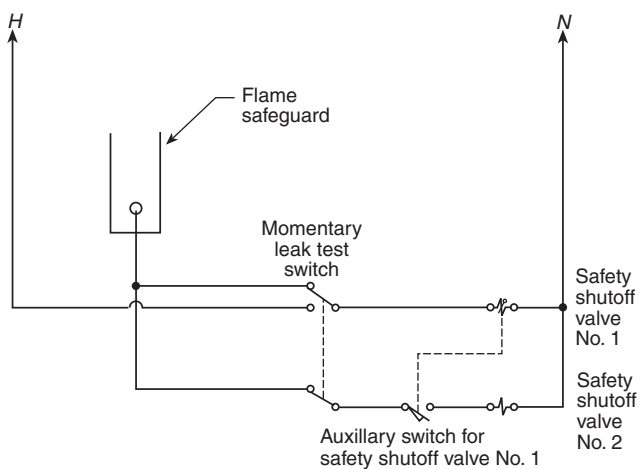
▲ FIGURE A.8.5.14(b) Example of a Wiring Diagram for Leak Test. [86:Figure A.7.4.10(b)]
