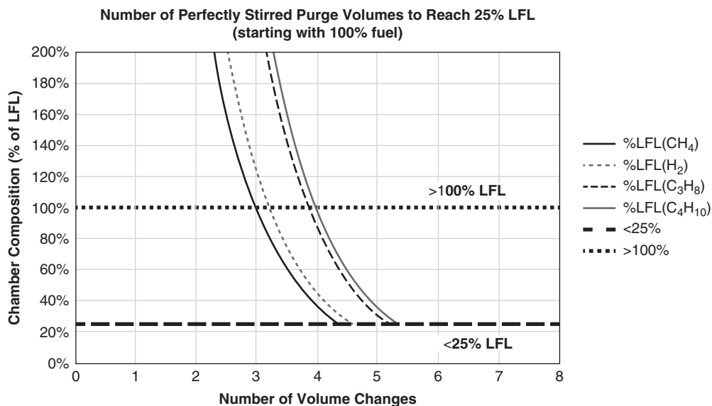
FIGURE A.9.5.1.1(1) Composition Profile for Four Fuel Gases Undergoing Fresh-Air Purging.
