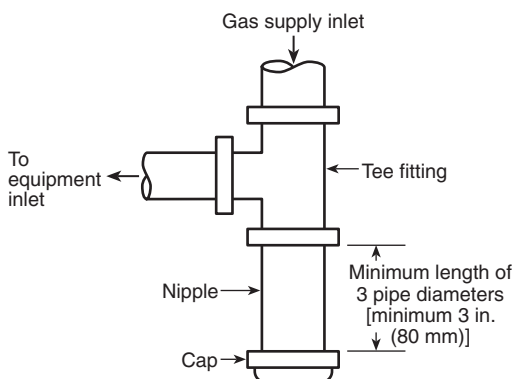
FIGURE 6.2.7.2 Method of Installing a Tee-Fitting Sediment Trap.
