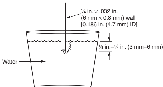
▲ FIGURE A.8.5.14(c) Leak Test for a Safety Shutoff Valve. [86:Figure A.7.4.10(c)]
