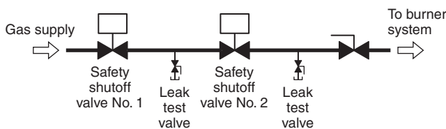
▲ FIGURE A.8.5.14(a) Example of a Gas Piping Diagram for Leak Test. [86:Figure A.7.4.10(a)]
