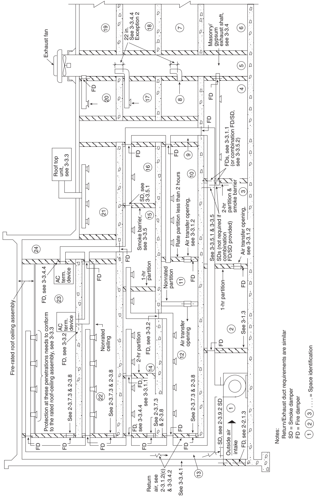
Figure A-3.3 Application of penetration requirements.
