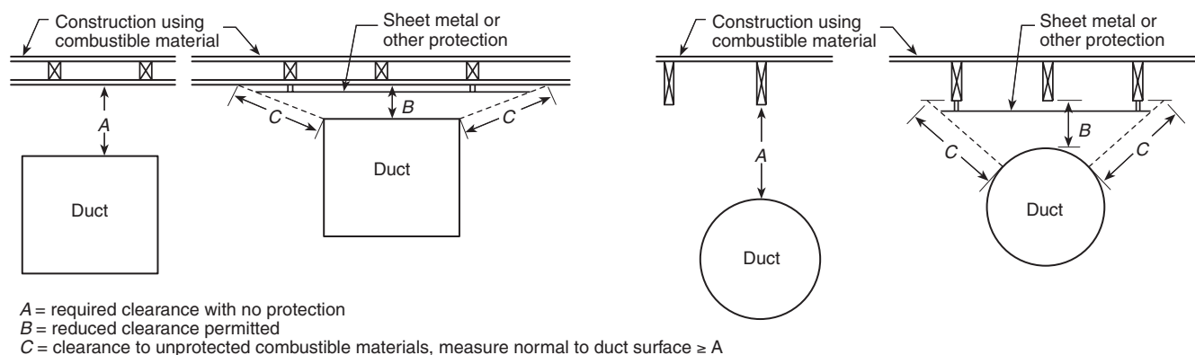
FIGURE 4.7.5.1 Extent of Protection Required to Reduce Clearances from Ducts.
