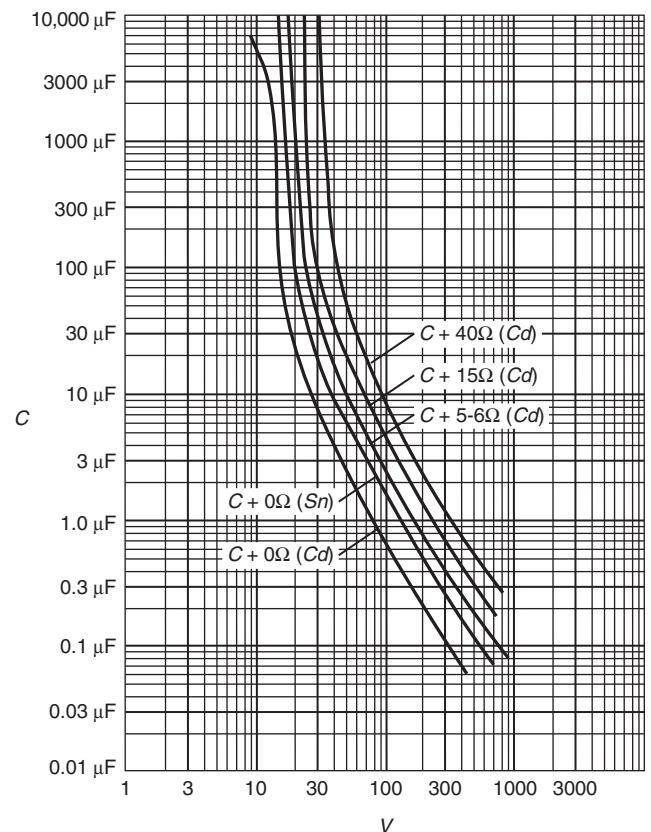
FIGURE 10.2.9.3(f) Capacitance Circuits Minimum Ignition Voltages. The Curves Correspond to Values of Current-limiting Resistance as Indicated. The Curve Marked S_n is Applicable Only Where Cadmium, Zinc, or Magnesium Can Be Excluded.
