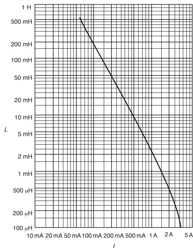
FIGURE 10.5.4.1(e) Inductance Circuits ( L > 1 \text{ mH} ): Minimum Igniting Currents at 24 V, Applicable Only to Circuits Where Cadmium, Zinc, or Magnesium Can Be Excluded.
