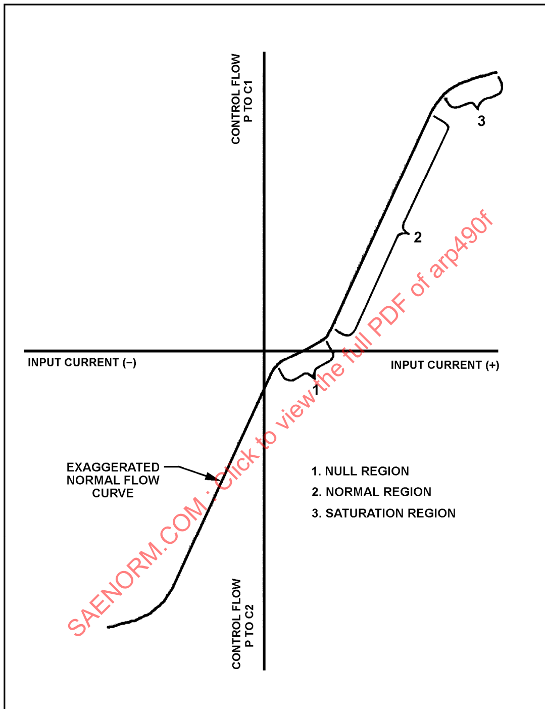
FIGURE 4 - OPERATING REGIONS
