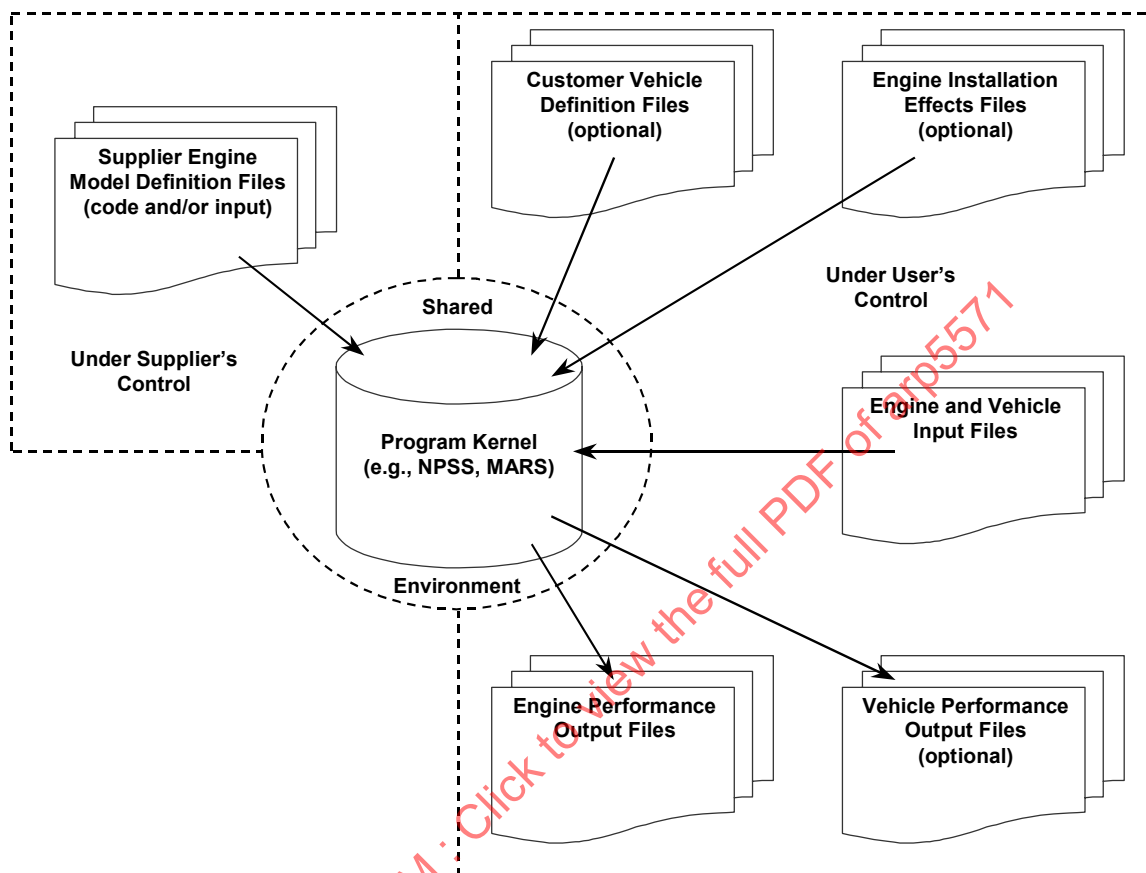
FIGURE 1 Shared/Restricted-Environment Architecture
