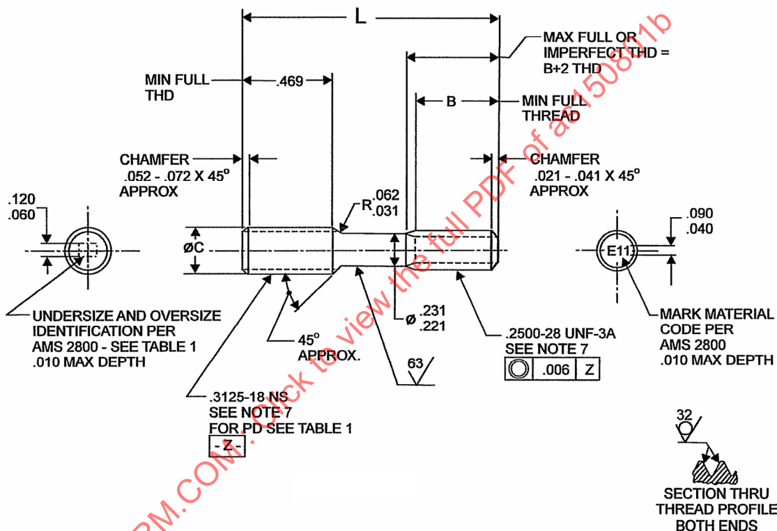
FIGURE 1 - STUD
