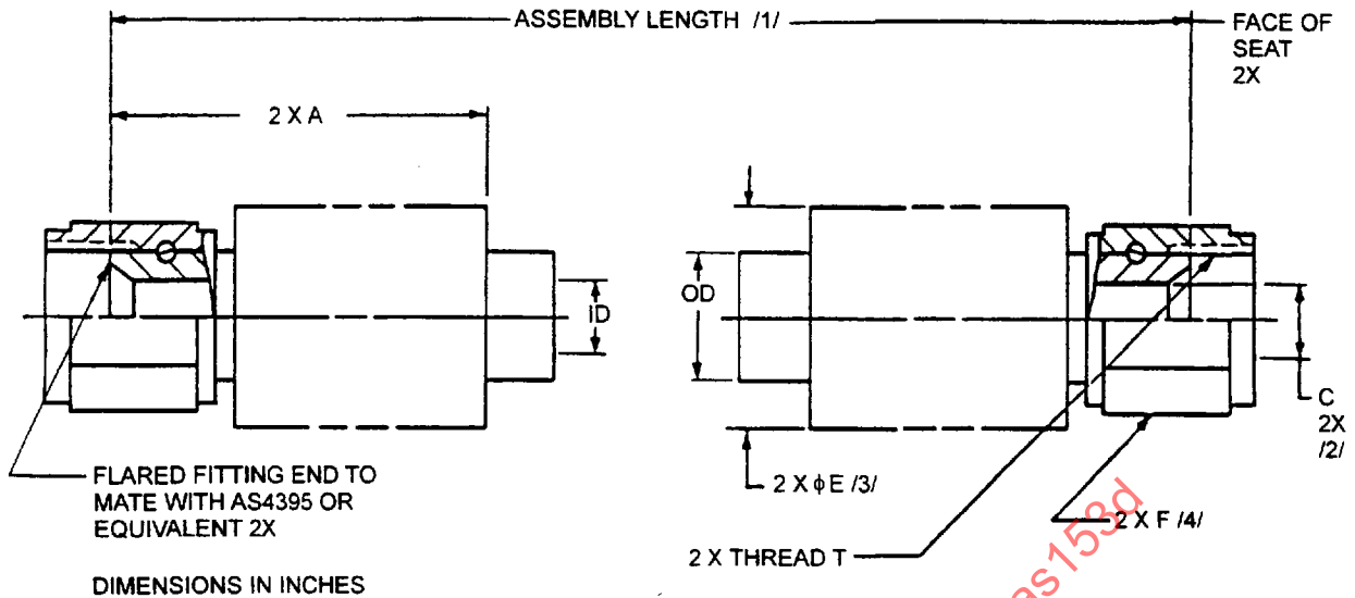
FIGURE 1 - HOSE AND FITTING DIMENSIONS
