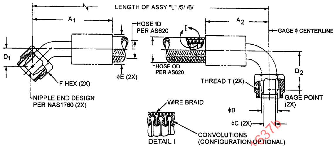
FIGURE 1 - HOSE ASSEMBLY
