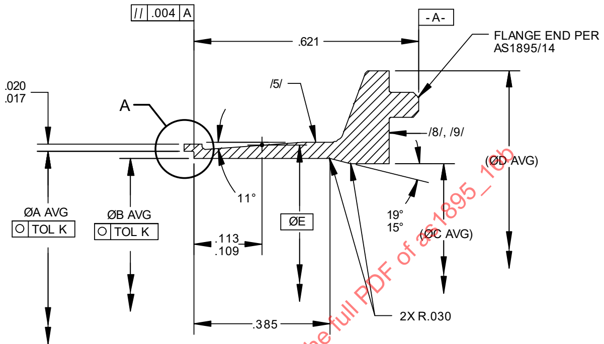
FIGURE 1 - TYPICAL SECTION
