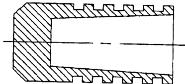
FIGURE 2 - AS3129 PLUG
