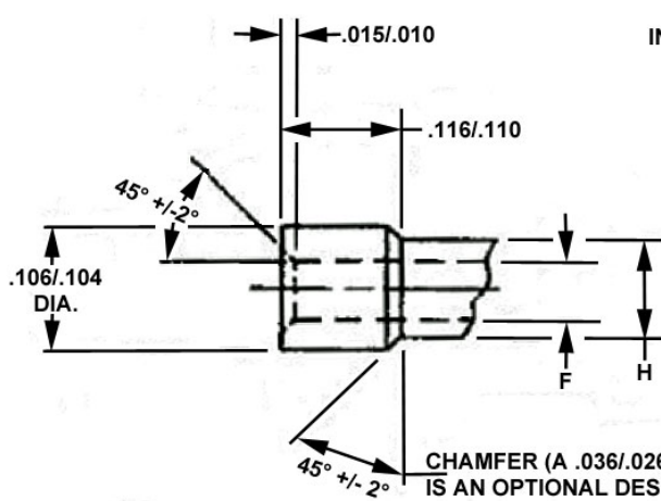
WIRE BARREL DESIGN BIN CODE 448 (SIZE 20)
