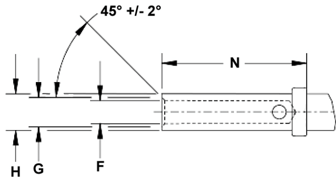
WIRE BARREL DESIGN 223 THROUGH 227 (SIZE 20 CONTACTS)
