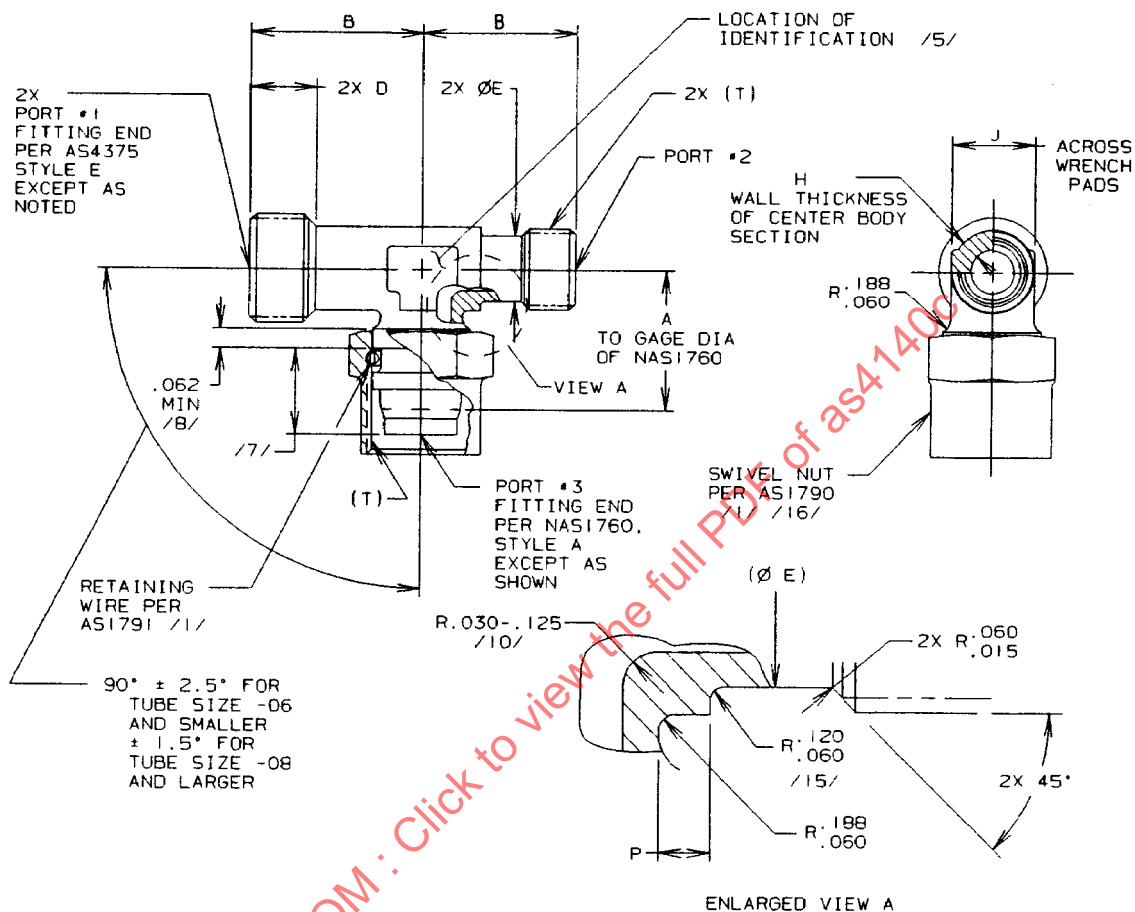
FIGURE 1 - FITTING ASSY, TEE, REDUCER, SWIVEL ON SIDE, REDUCED BODY, FLARELESS
