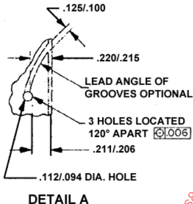
FIGURE 1A - PROTECTIVE COVER, RECEPTACLE (DETAIL A)
