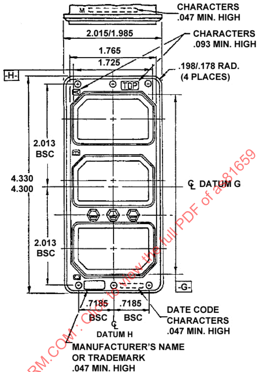
FIGURE 2 – CONNECTOR CONFIGURATIONS AND DIMENSIONS
