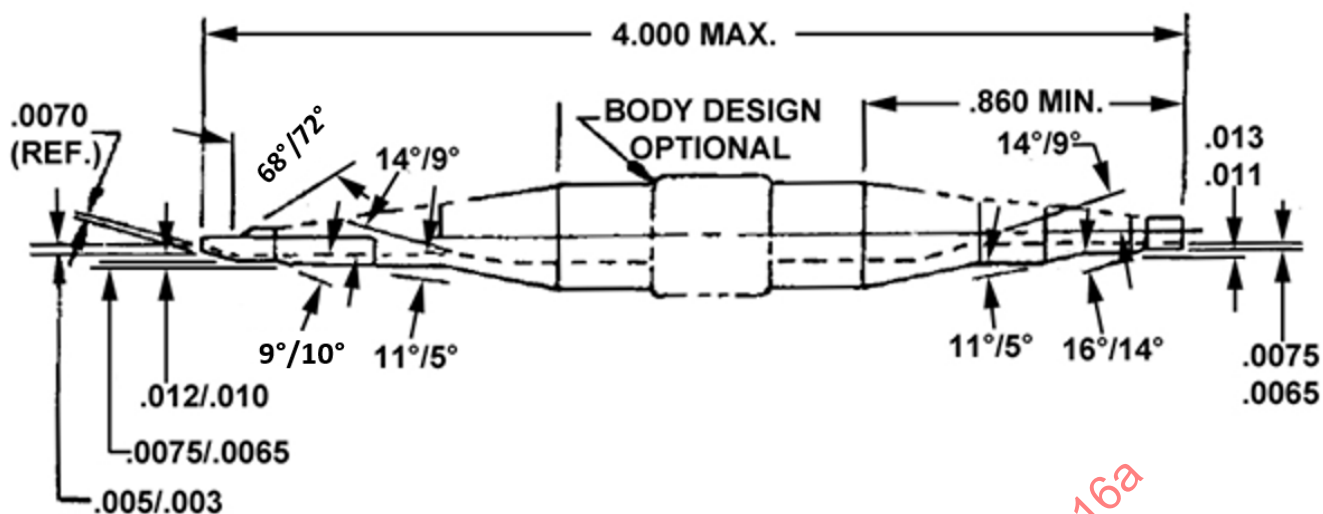
FIGURE 3 - INSTALLING AND REMOVAL TOOL (-04) (CONT.)
