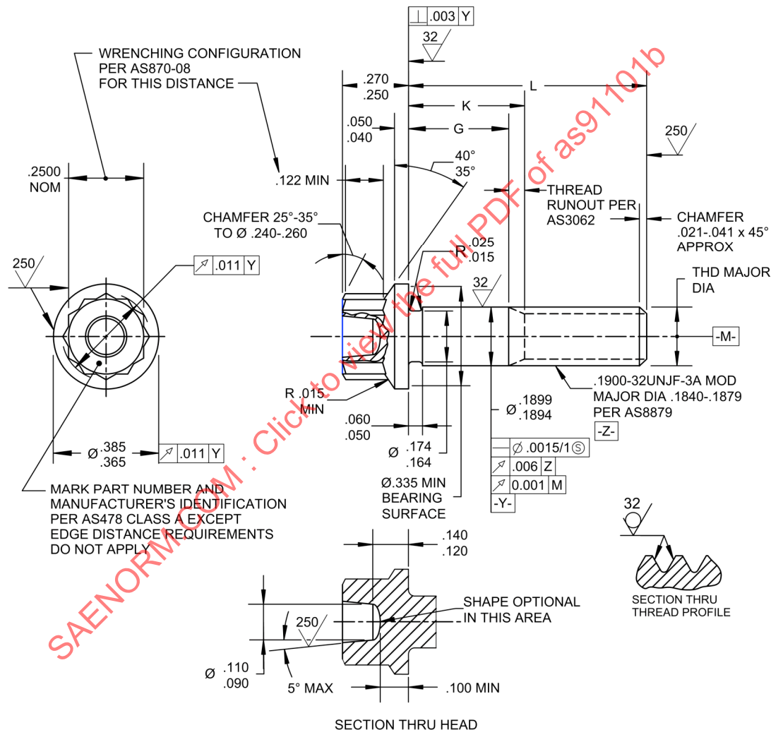
FIGURE 1 - BOLT
